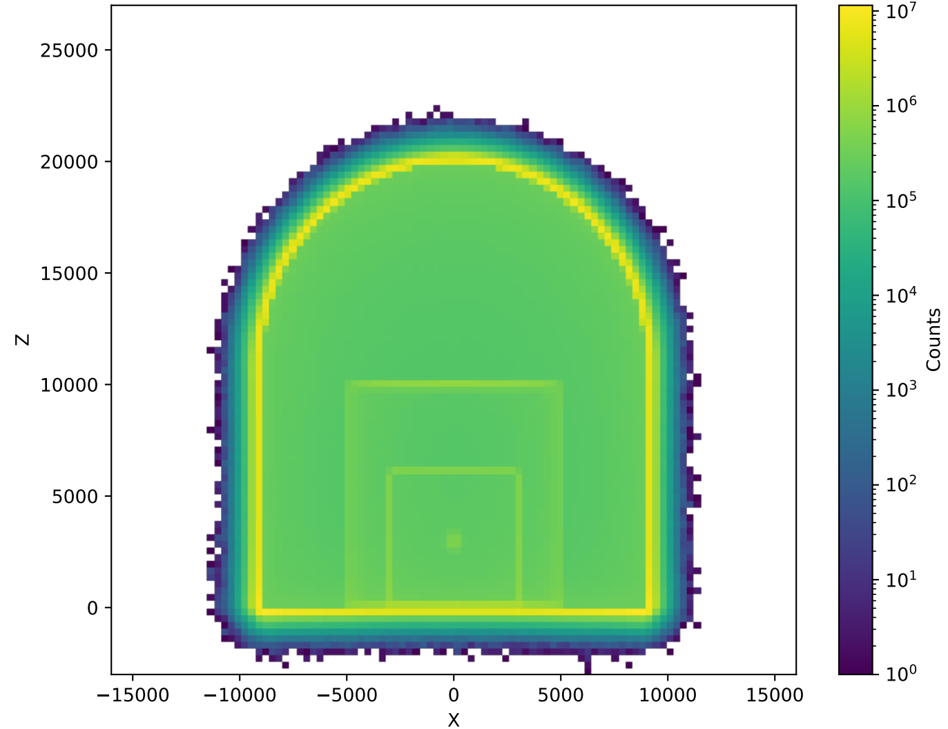
NeutronActivations (10cm, Polyethylen, 2.43e+09)
