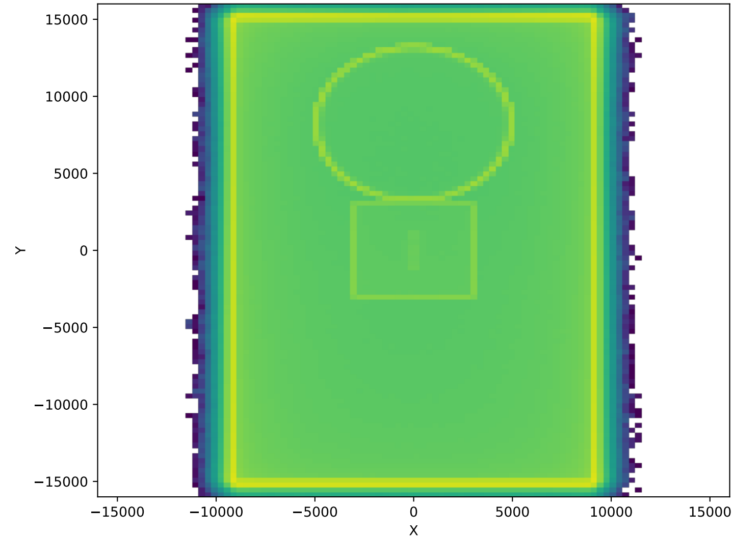
NeutronActivations (10cm, Polyethylen, 2.43e+09)
