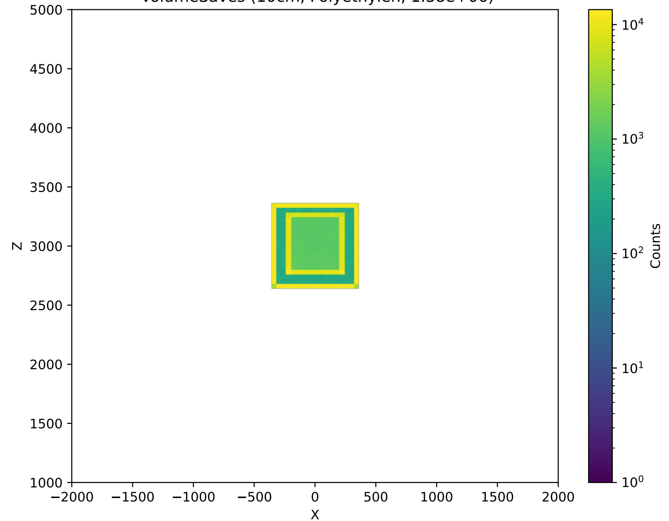
VolumeSaves (10cm, Polyethylen, 1.38e+06)
