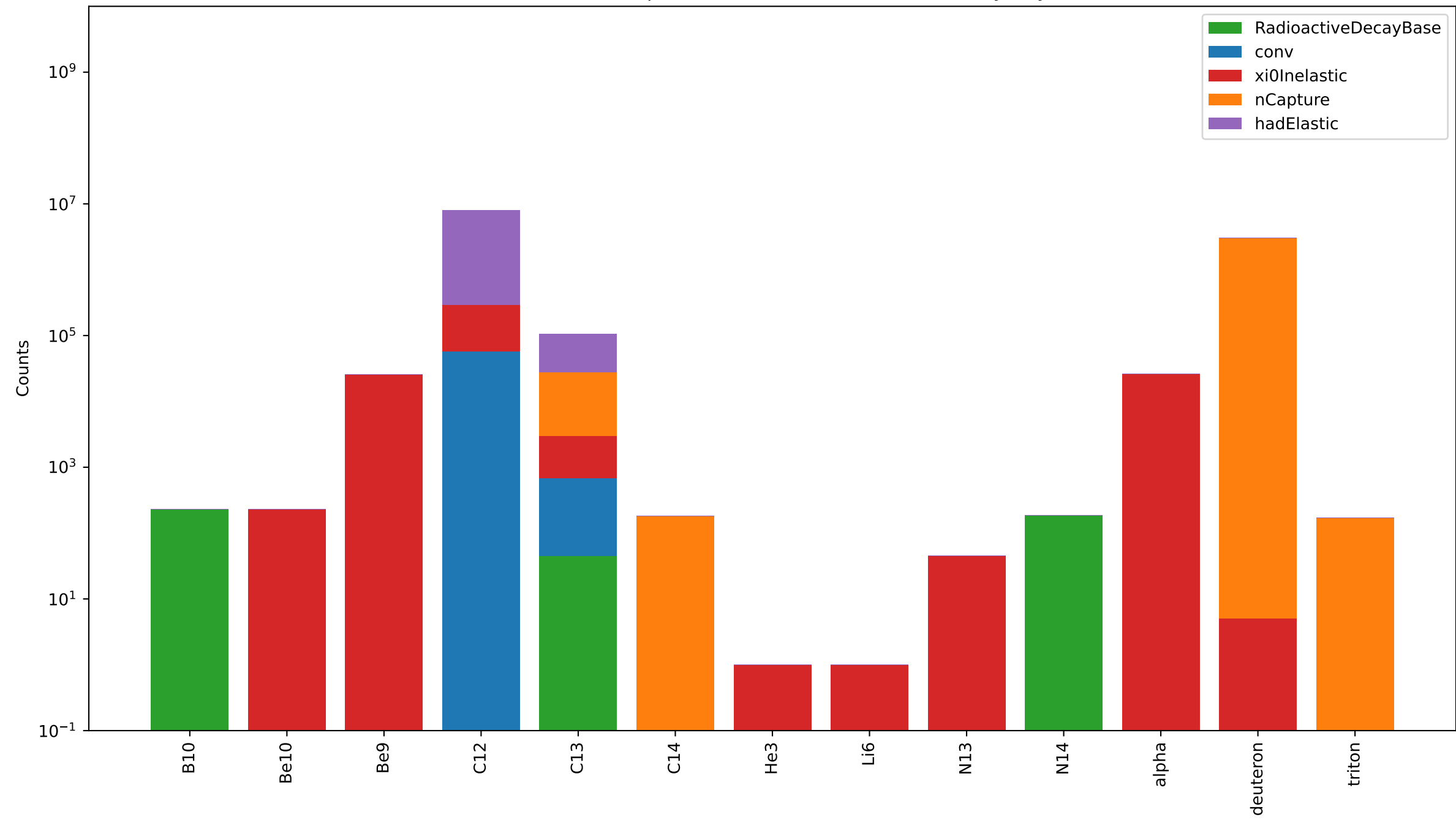
Neutron activation products in the Absorber (10cm Polyethylen)
