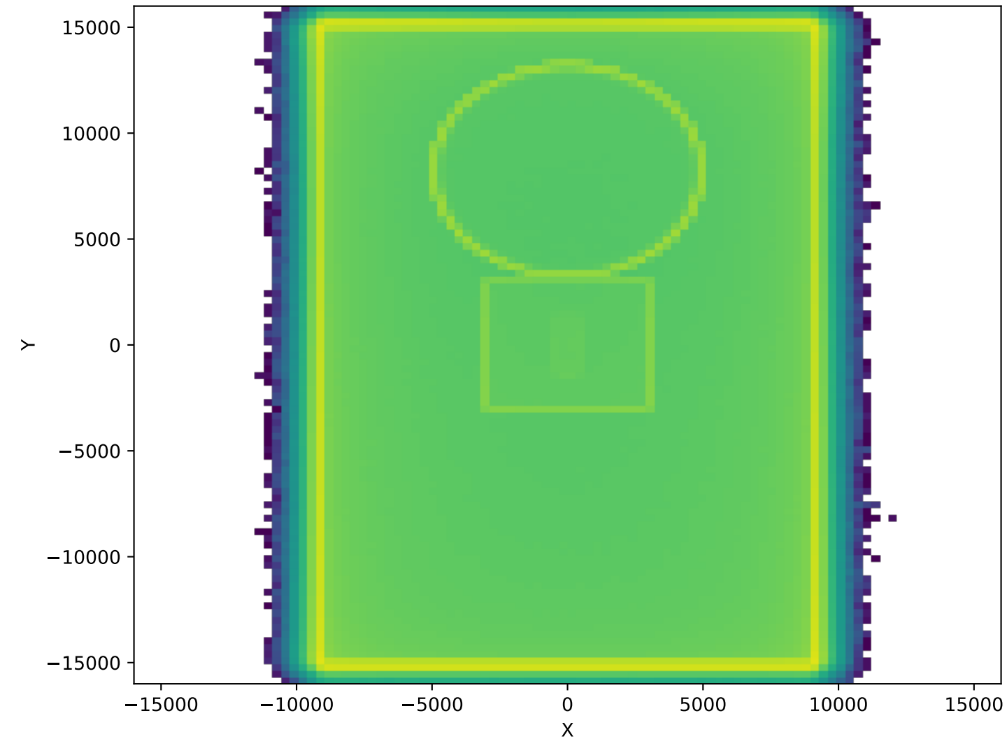
NeutronActivations (20cm, Polyethylen, 2.43e+09)
