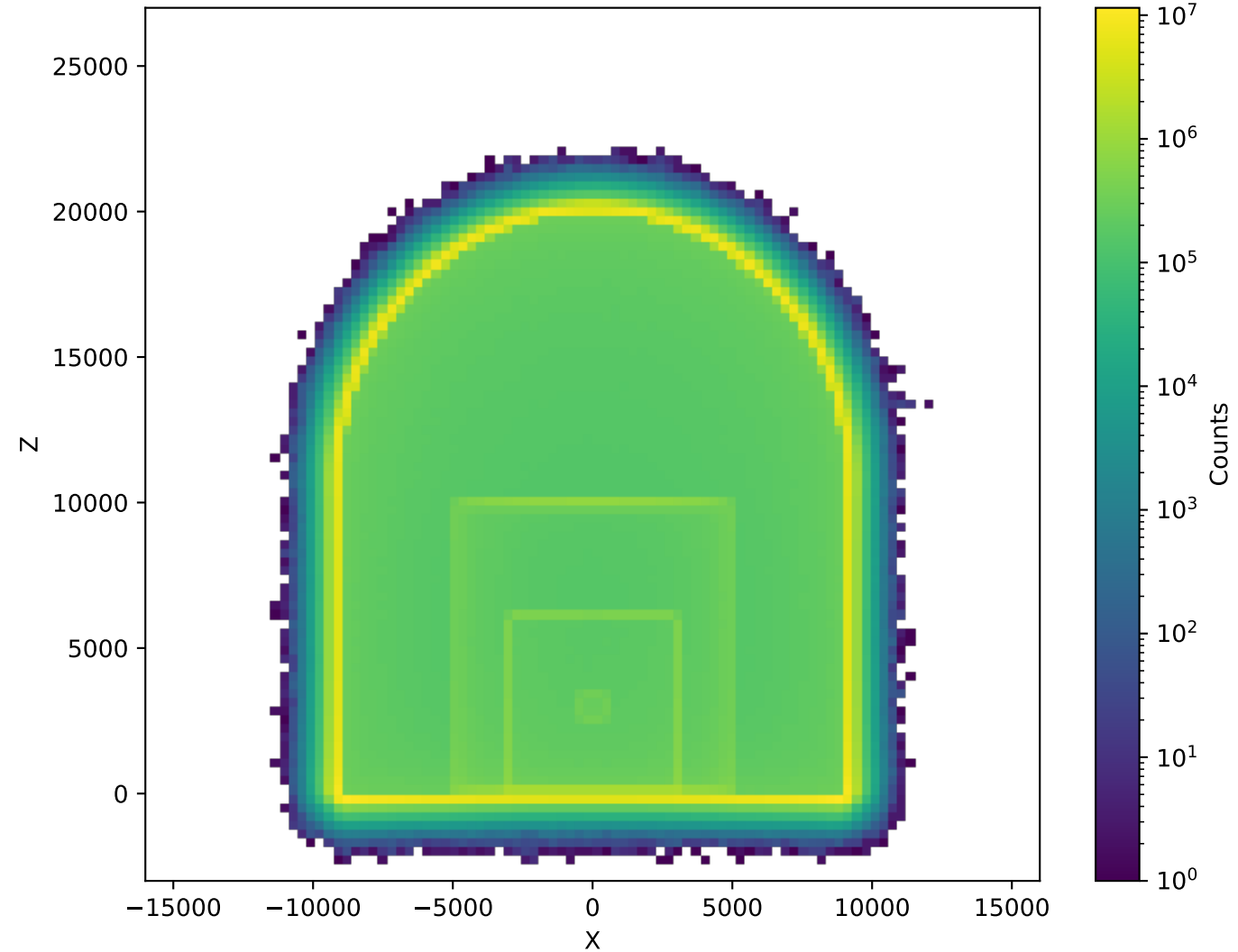
NeutronActivations (20cm, Polyethylen, 2.43e+09)
