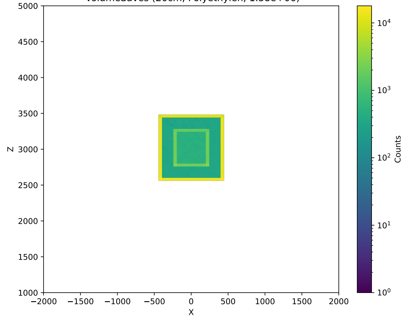
VolumeSaves (20cm, Polyethylen, 1.38e+06)
