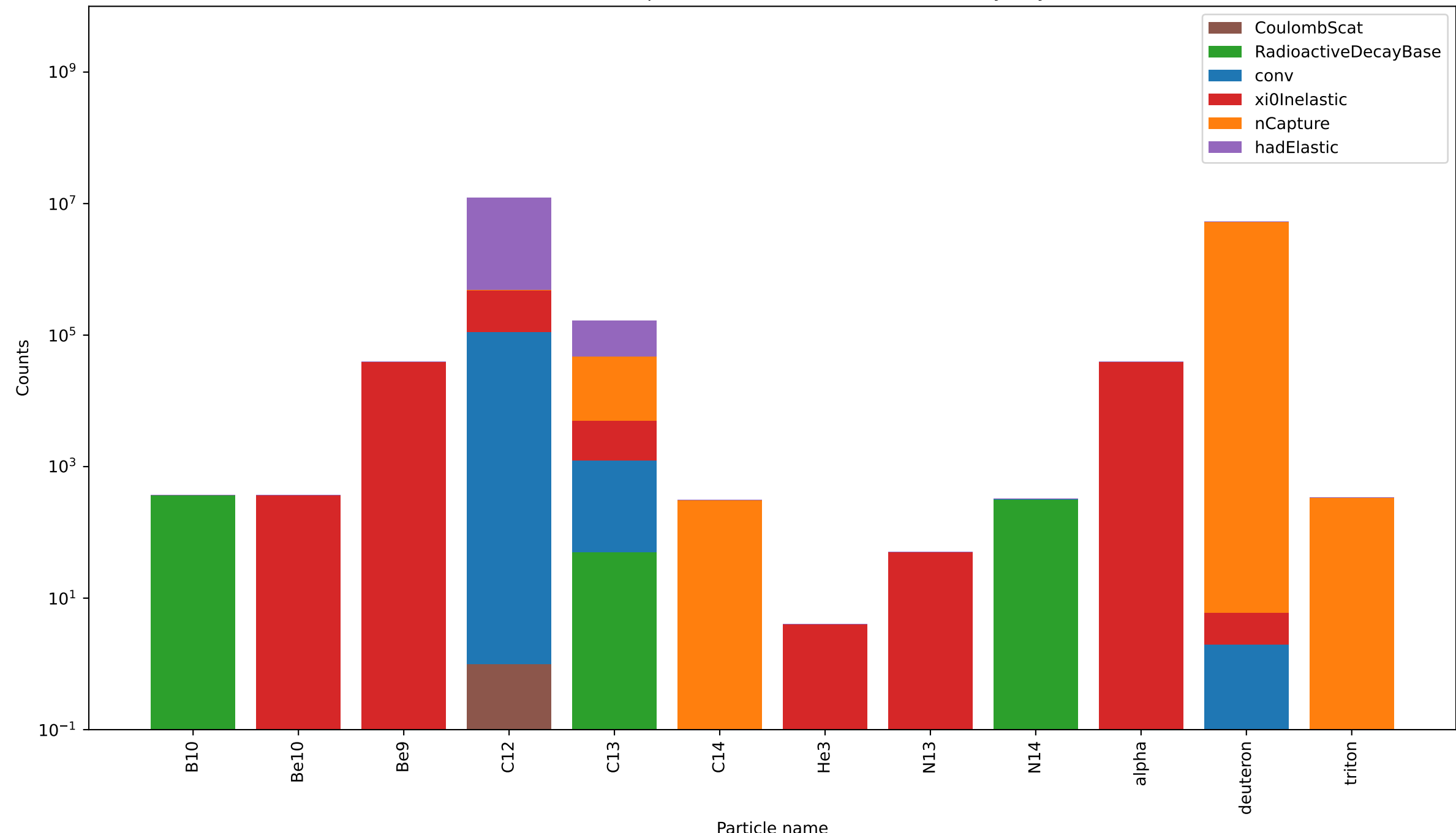
Neutron activation products in the Absorber (20cm Polyethylen)
