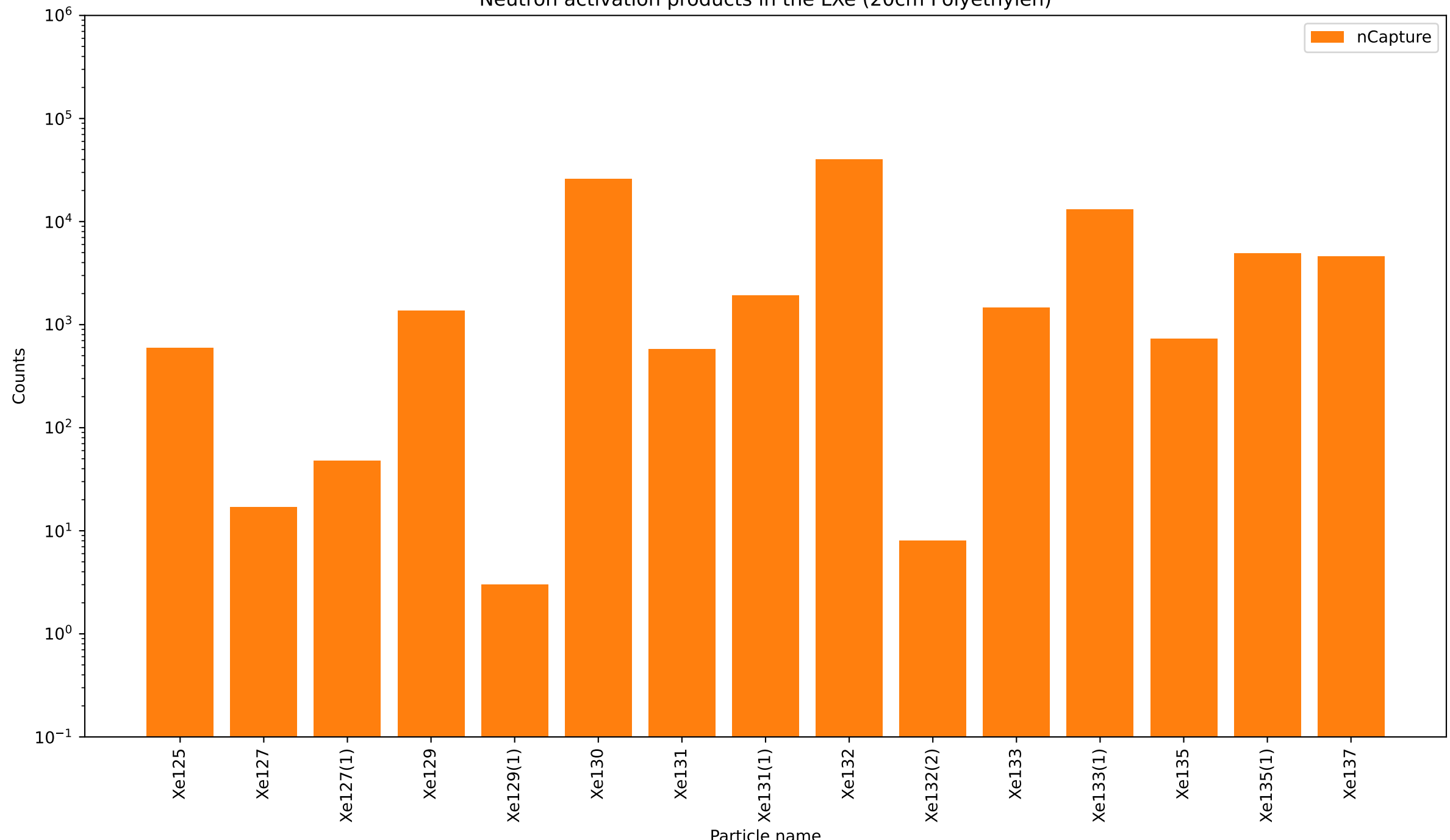
Neutron activation products in the LXe (20cm Polyethylen)
