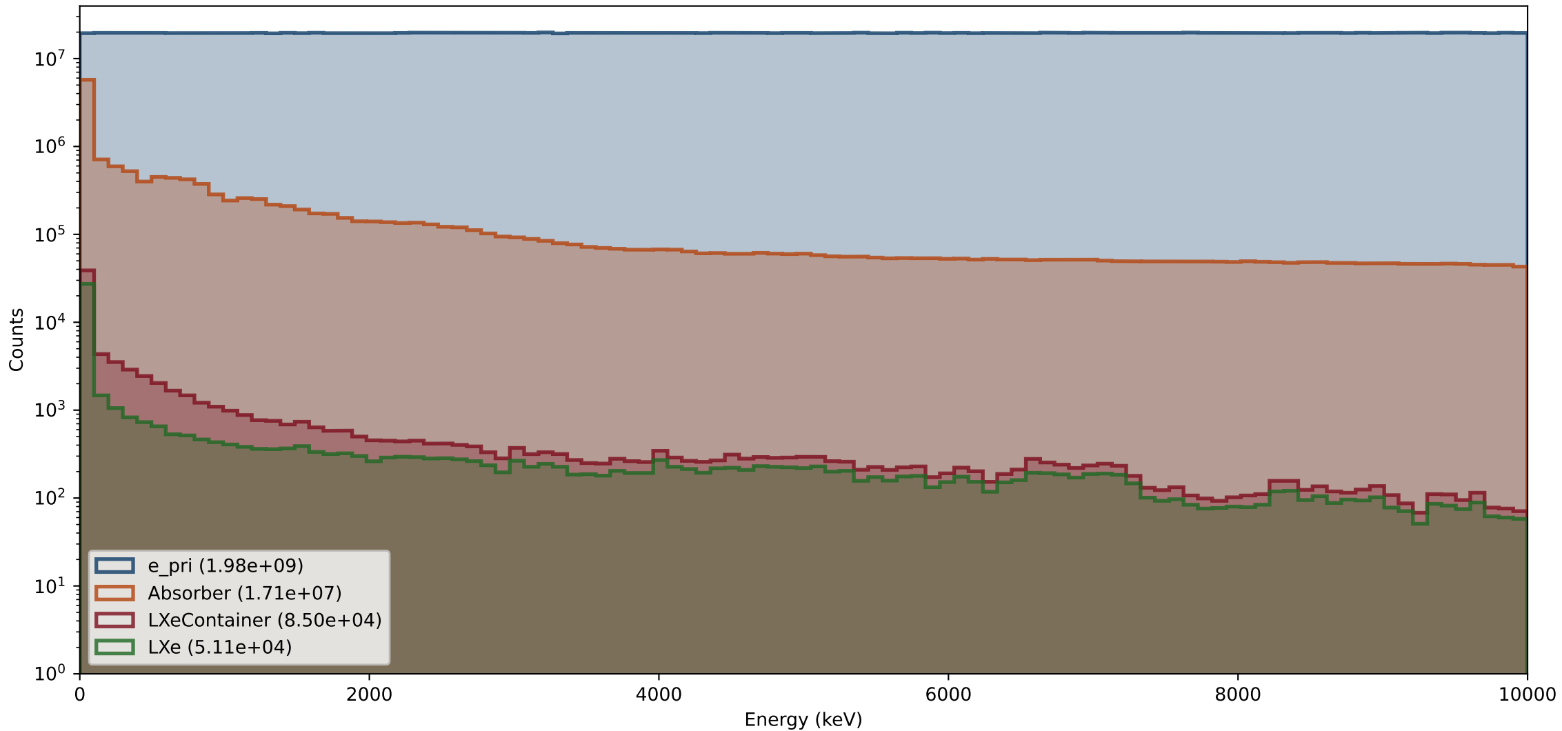
Energy distribution entering different volumes (30cm Polyethylen)
