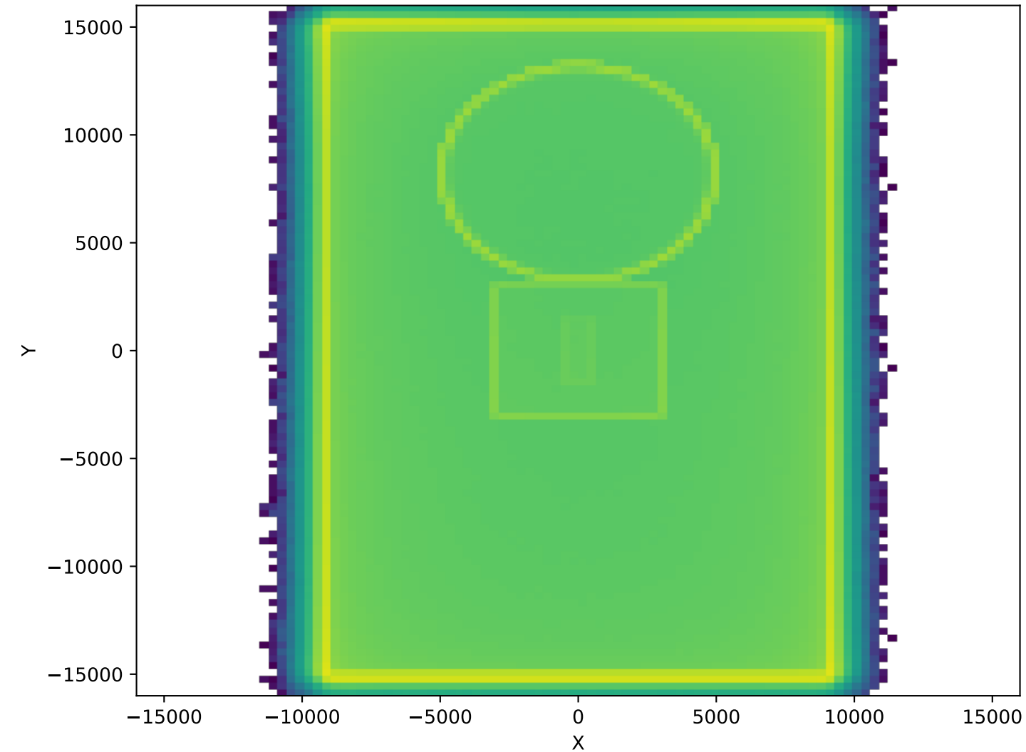
NeutronActivations (30cm, Polyethylen, 2.43e+09)
