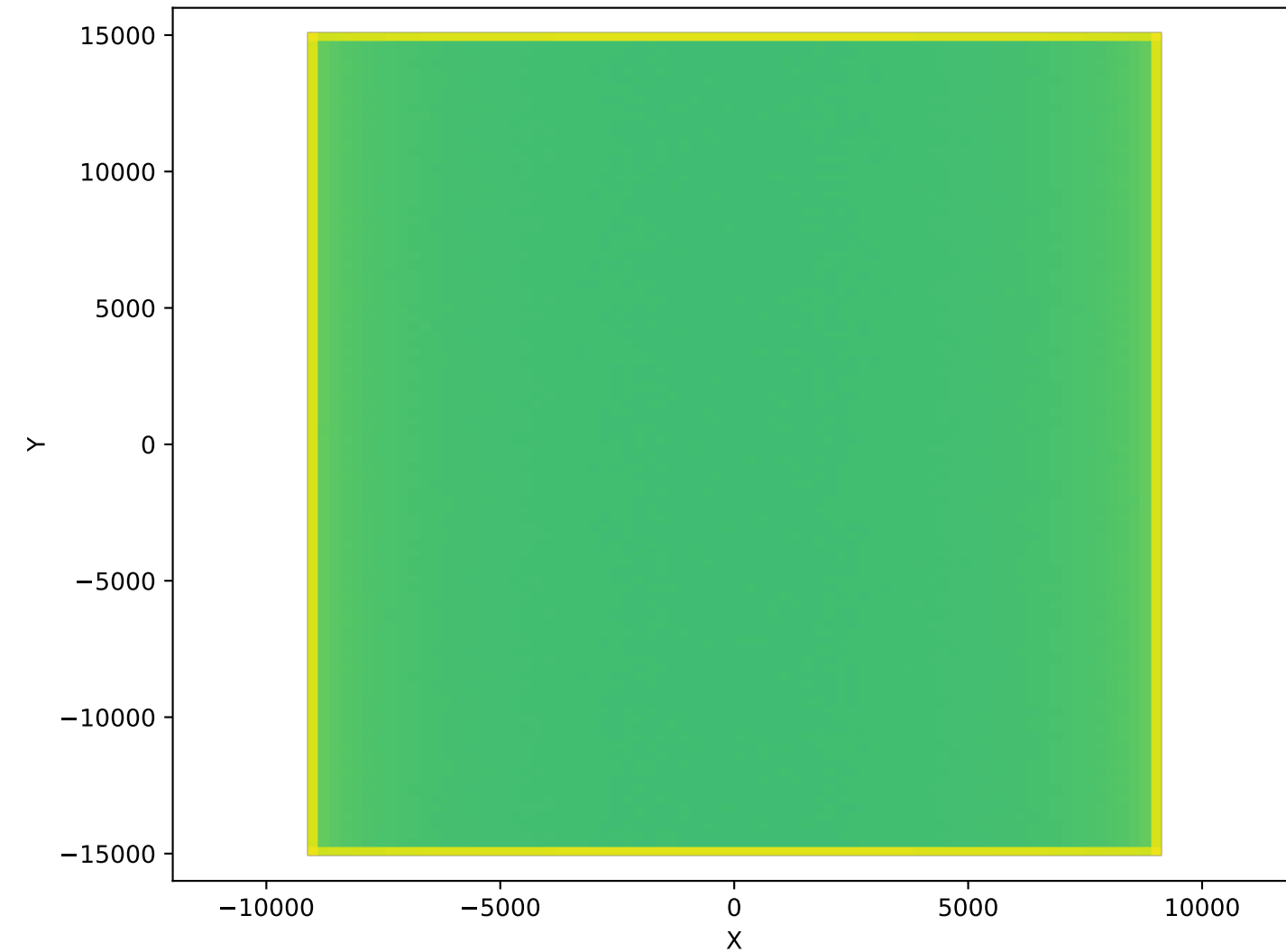
PrimaryNeutrons (30cm, Polyethylen, 1.98e+08)
