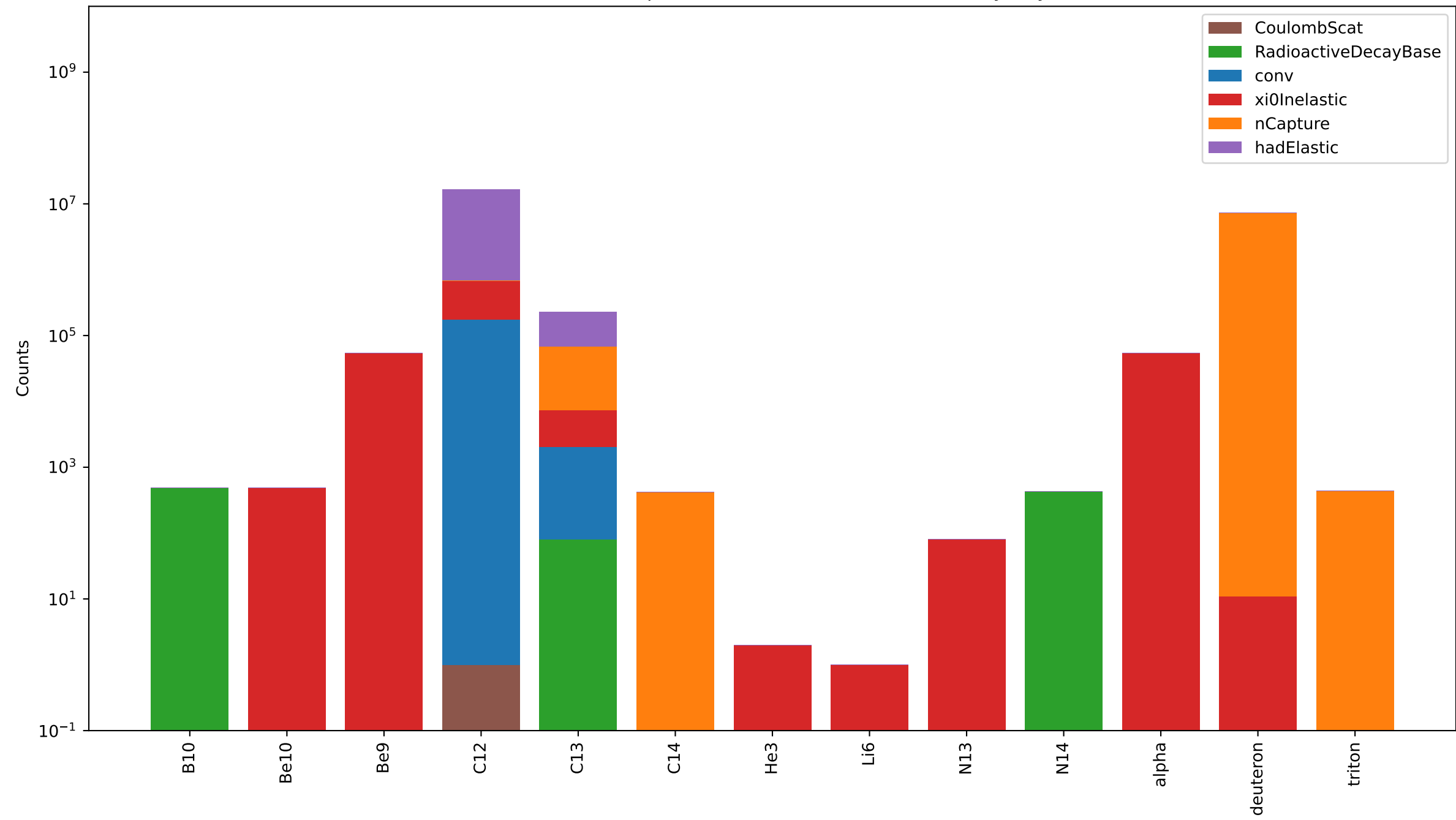
Neutron activation products in the Absorber (30cm Polyethylen)
