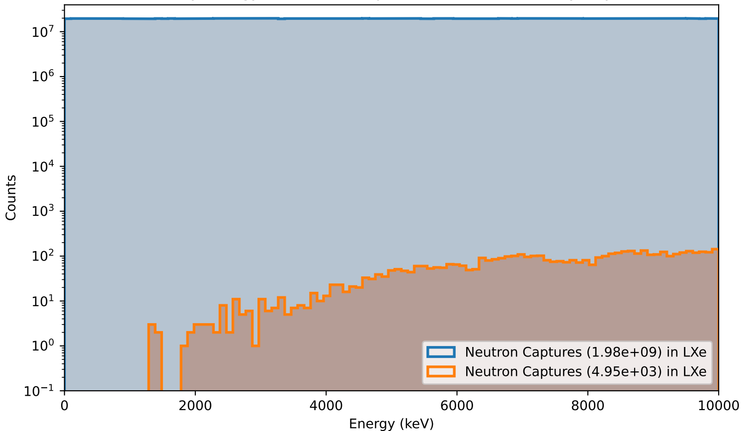
Primary energy of Neutron Captures in LXe (40cm,Polyethylen)
