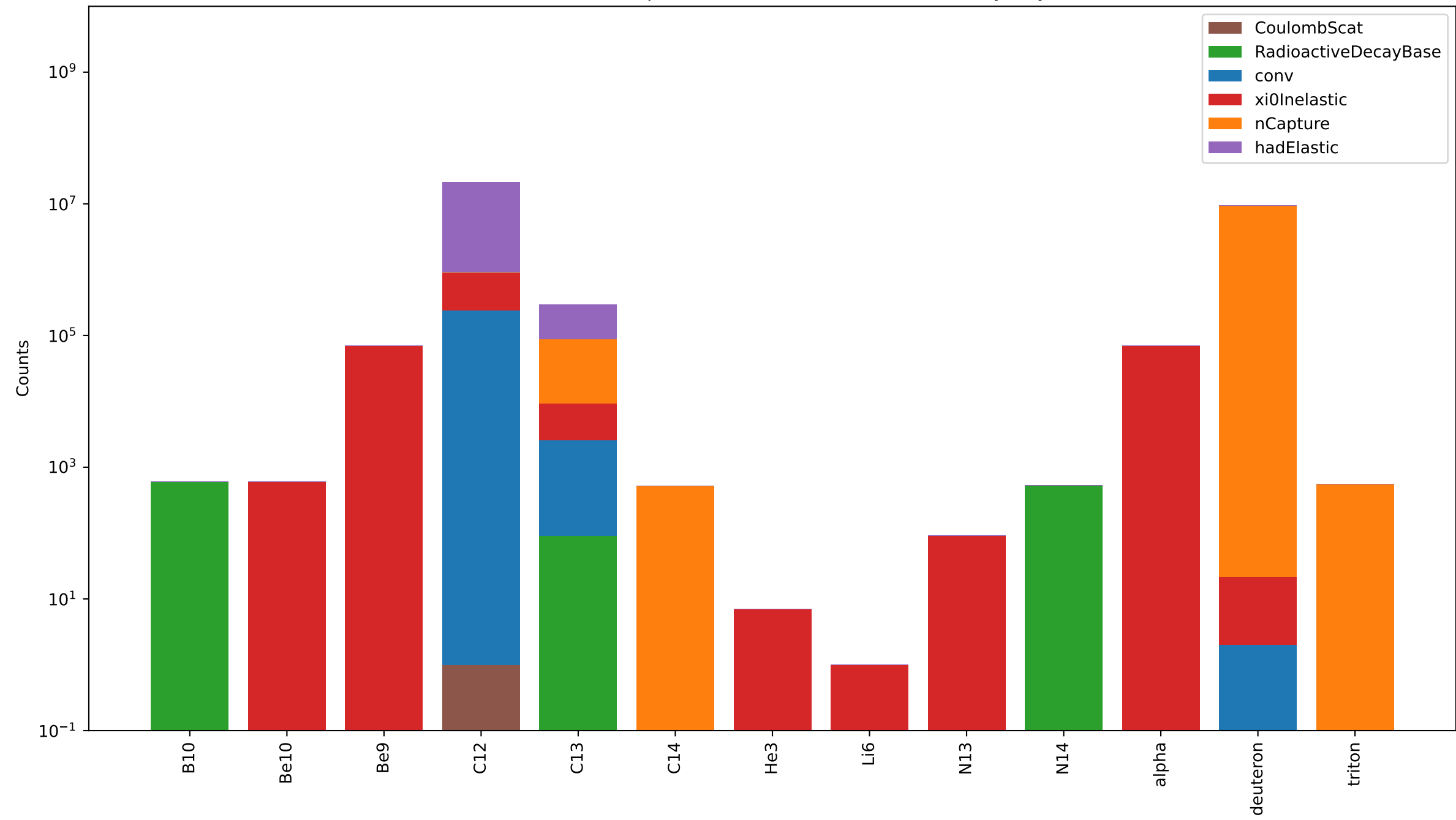
Neutron activation products in the Absorber (40cm Polyethylen)
