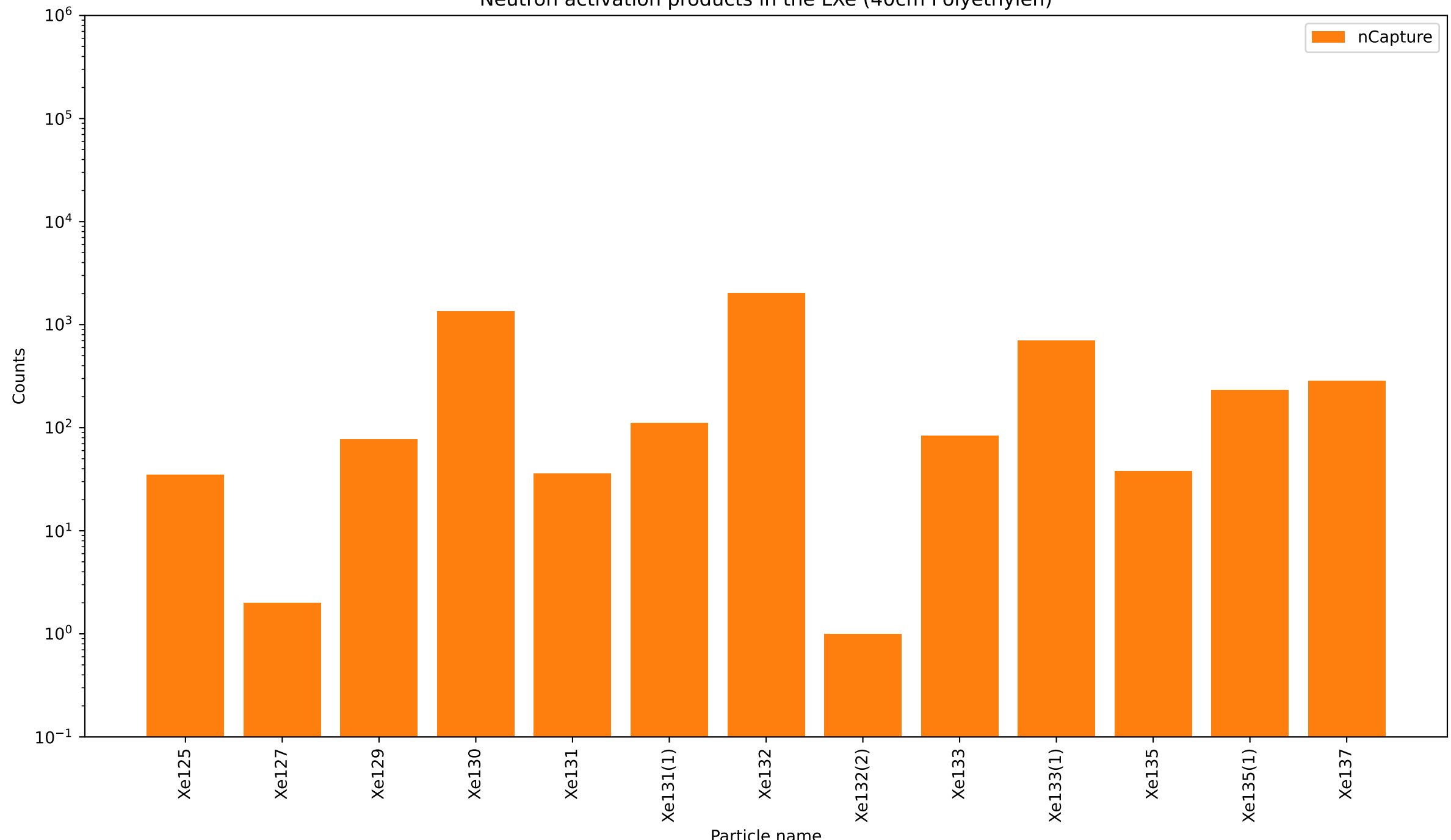
Neutron activation products in the LXe (40cm Polyethylen)
