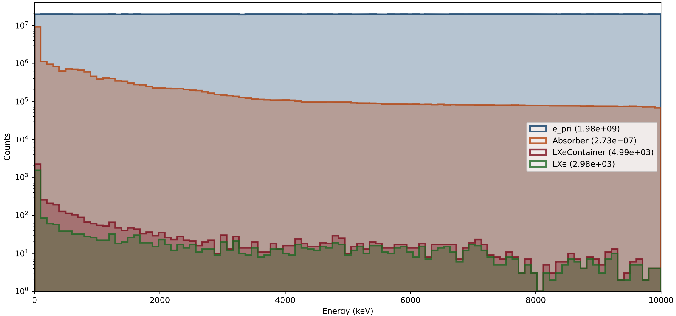
Energy distribution entering different volumes (50cm Polyethylen)
