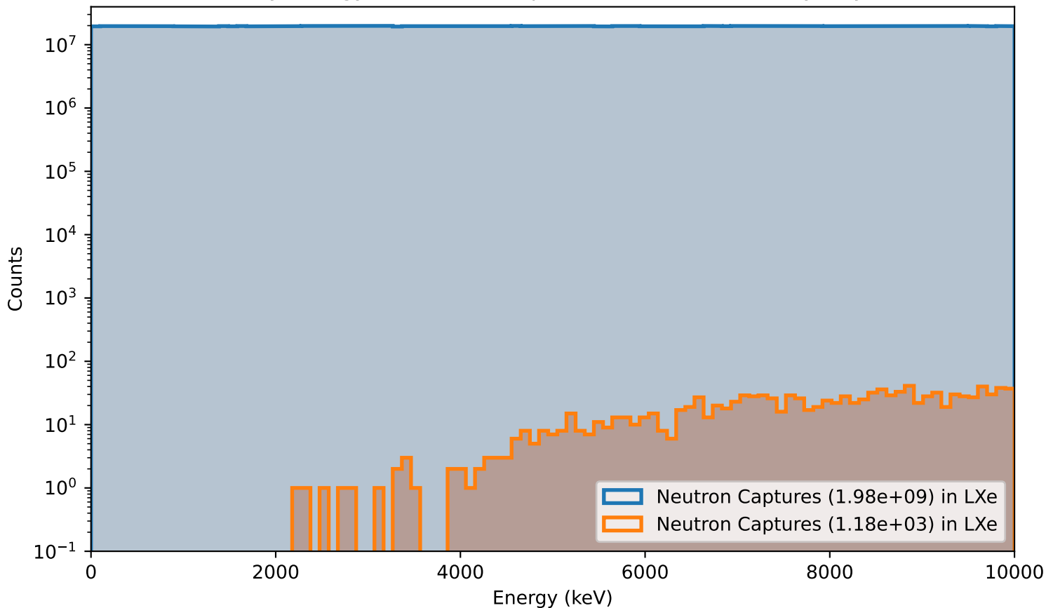
Primary energy of Neutron Captures in LXe (50cm,Polyethylen)
