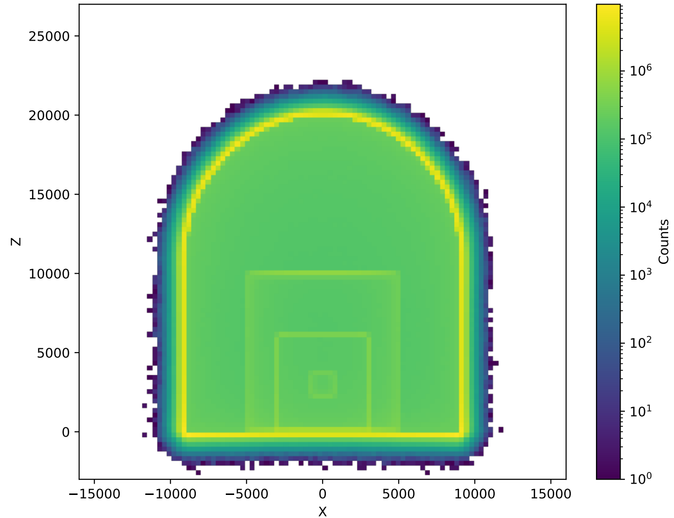
NeutronActivations (50cm, Polyethylen, 2.02e+09)
