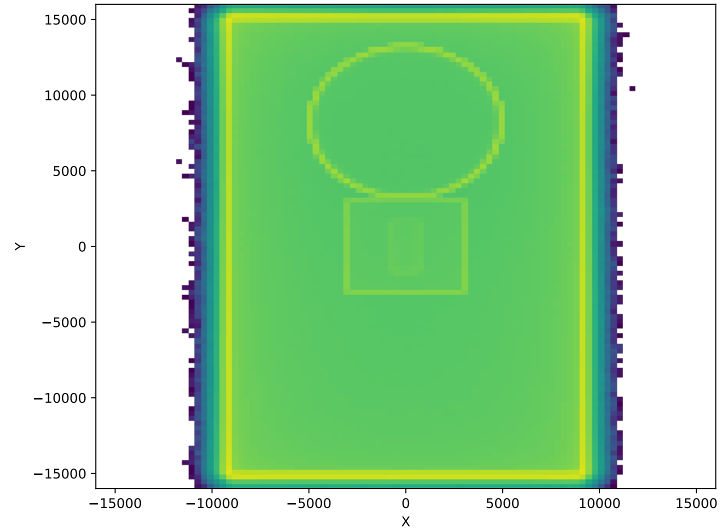
NeutronActivations (50cm, Polyethylen, 2.02e+09)
