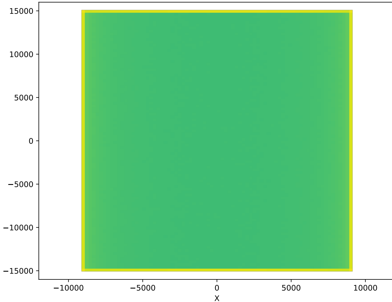
PrimaryNeutrons (50cm, Polyethylen, 1.65e+08)
