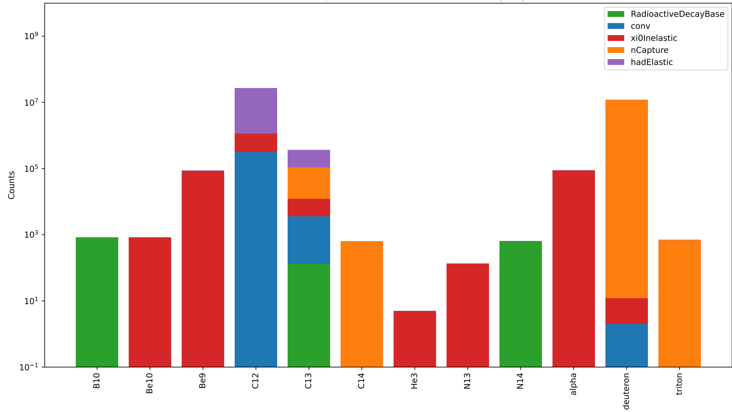
Neutron activation products in the Absorber (50cm Polyethylen)
