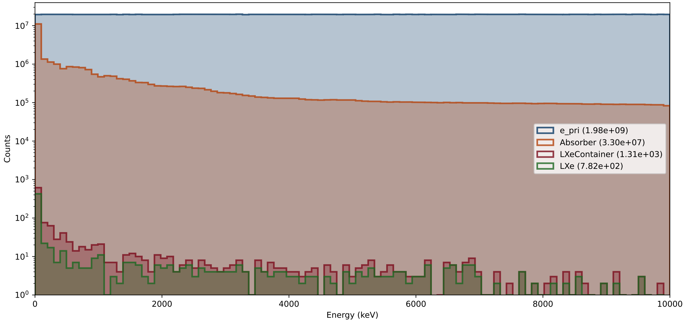
Energy distribution entering different volumes (60cm Polyethylen)
