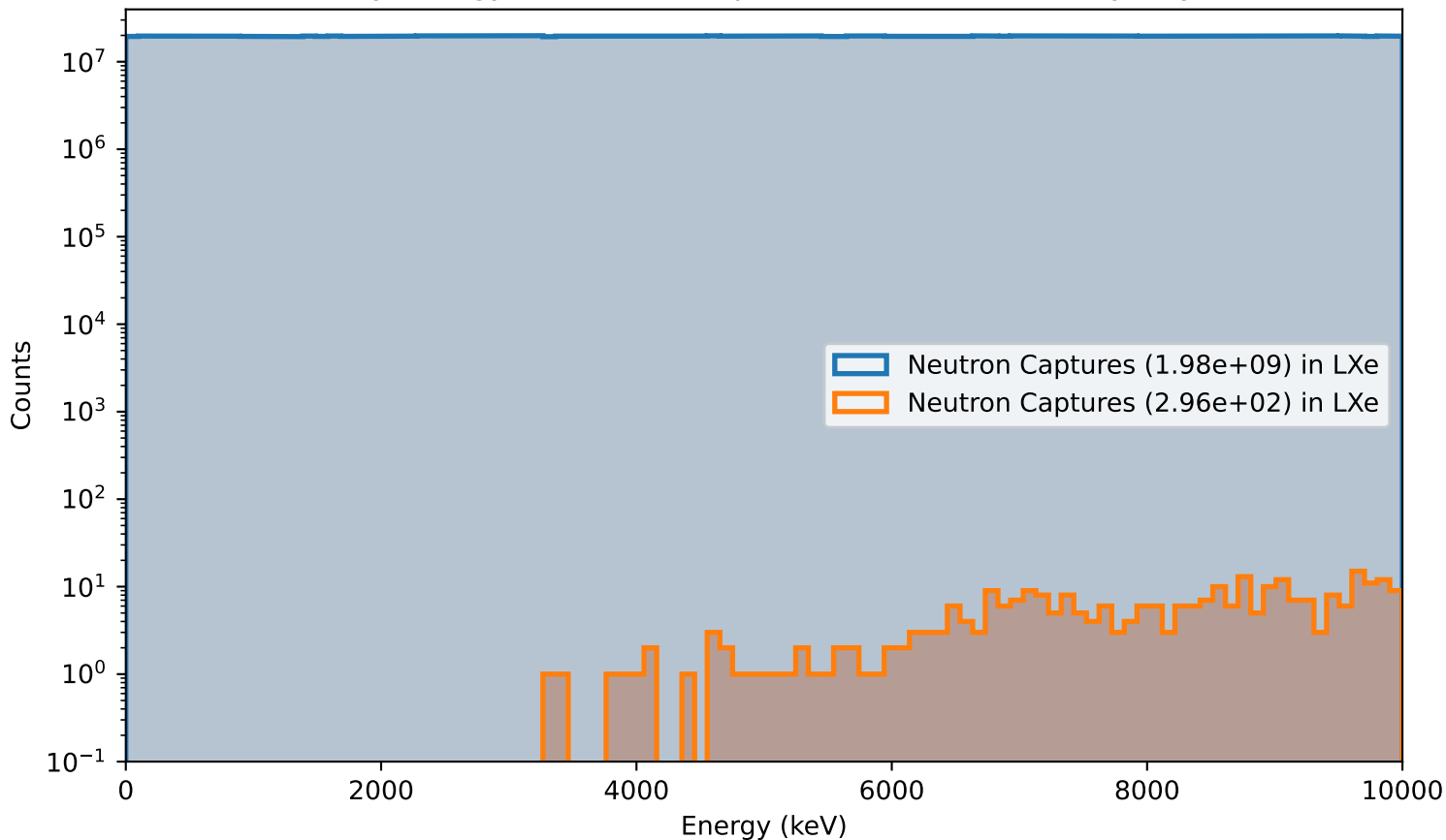
Primary energy of Neutron Captures in LXe (60cm,Polyethylen)
