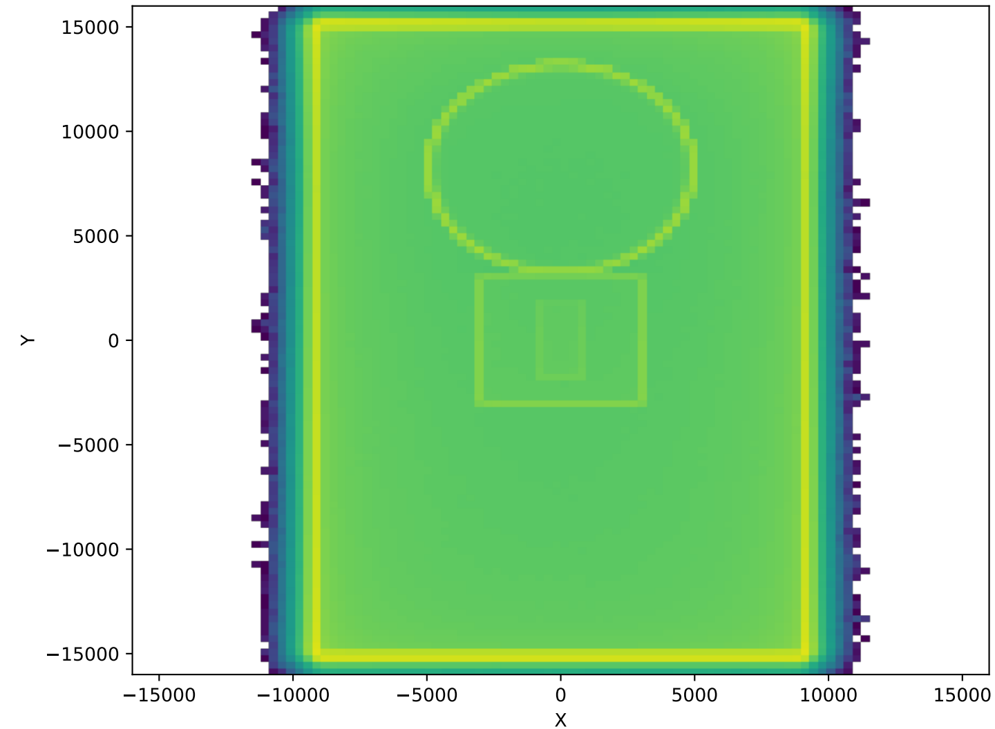
NeutronActivations (60cm, Polyethylen, 2.42e+09)
