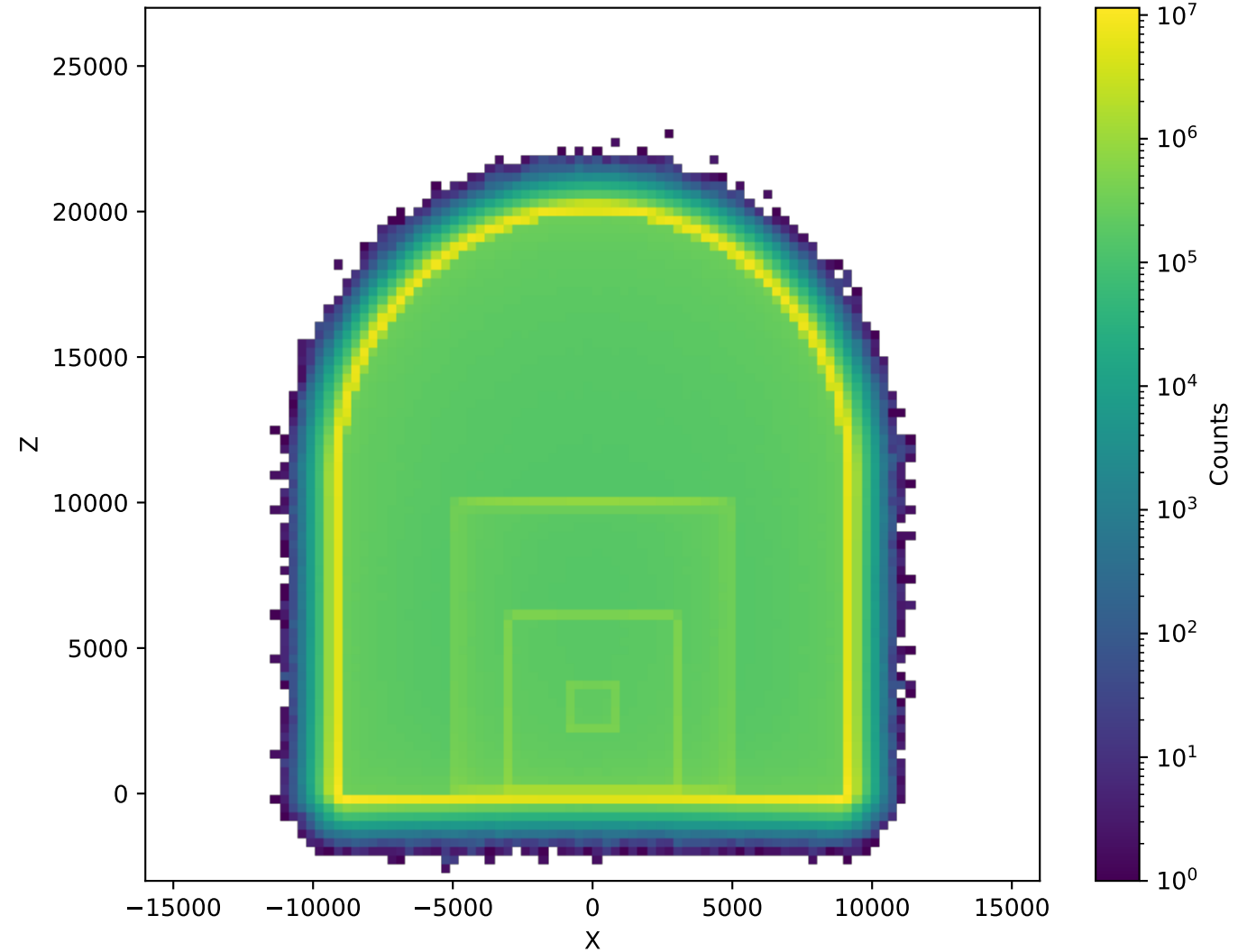
NeutronActivations (60cm, Polyethylen, 2.42e+09)
