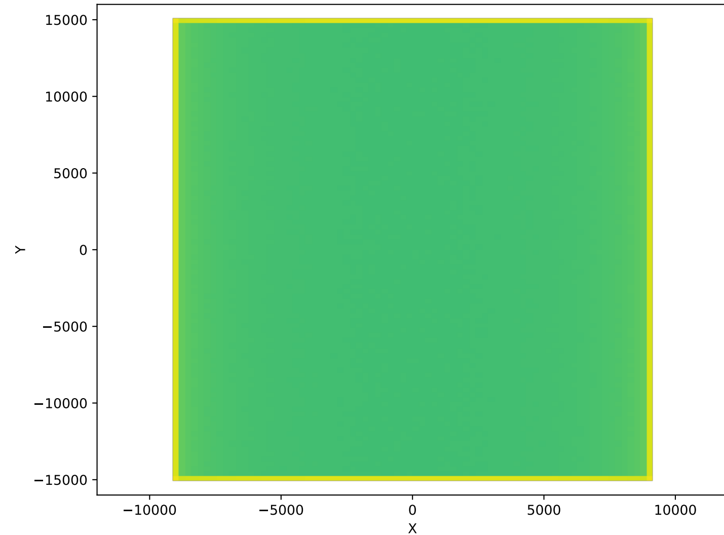
PrimaryNeutrons (60cm, Polyethylen, 1.98e+08)
