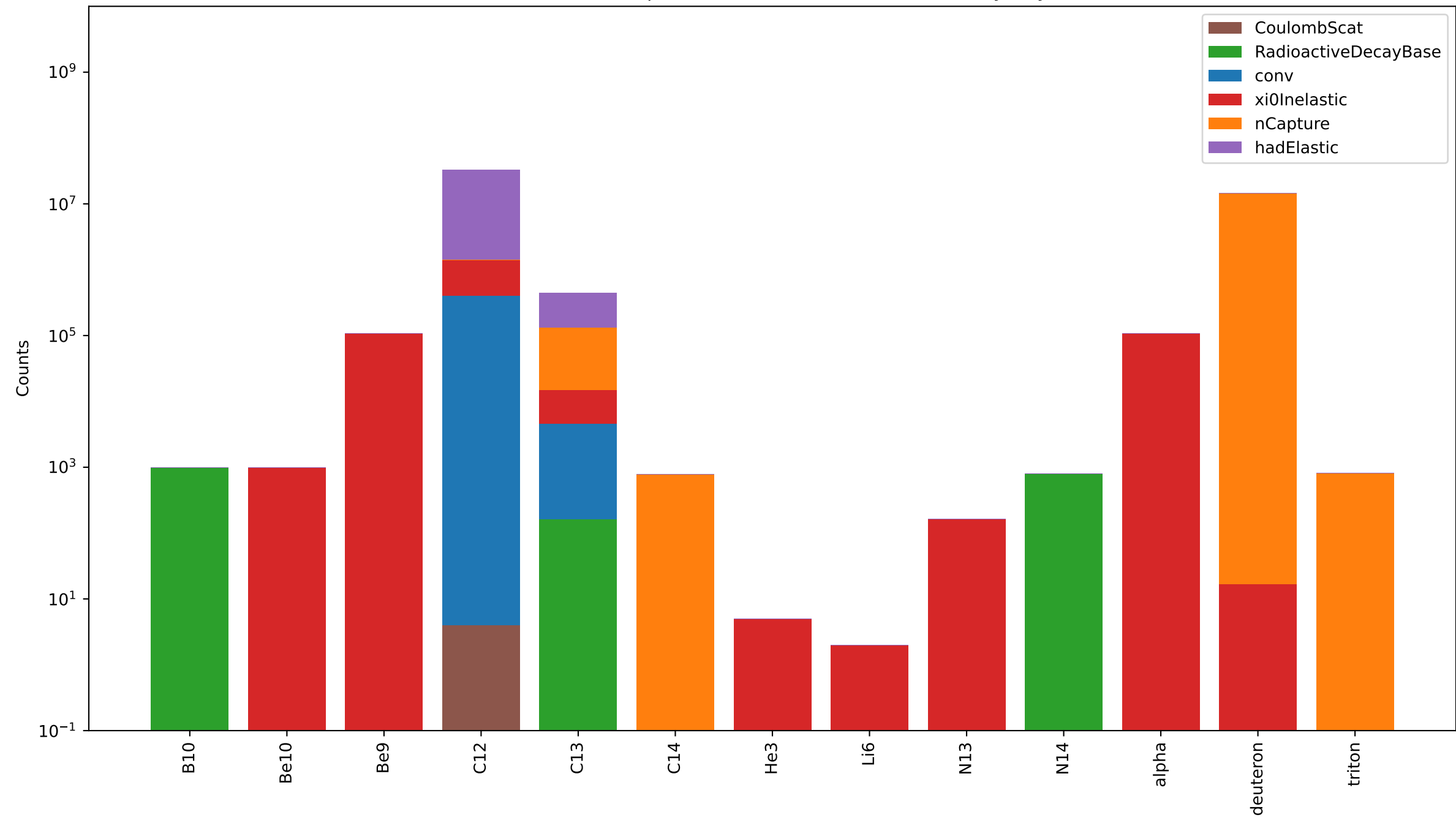
Neutron activation products in the Absorber (60cm Polyethylen)
