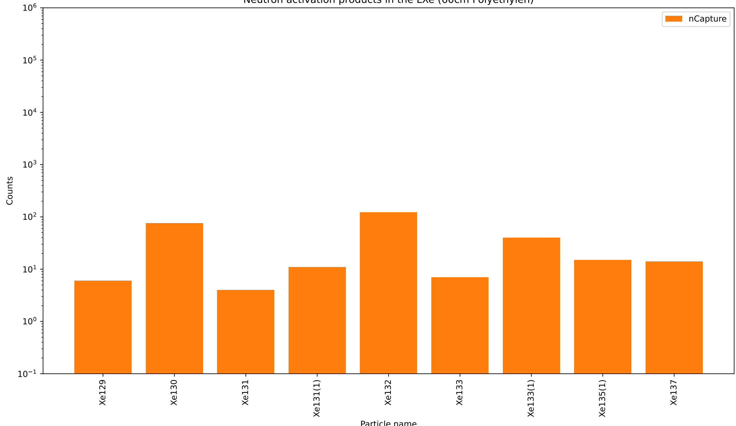
Neutron activation products in the LXe (60cm Polyethylen)
