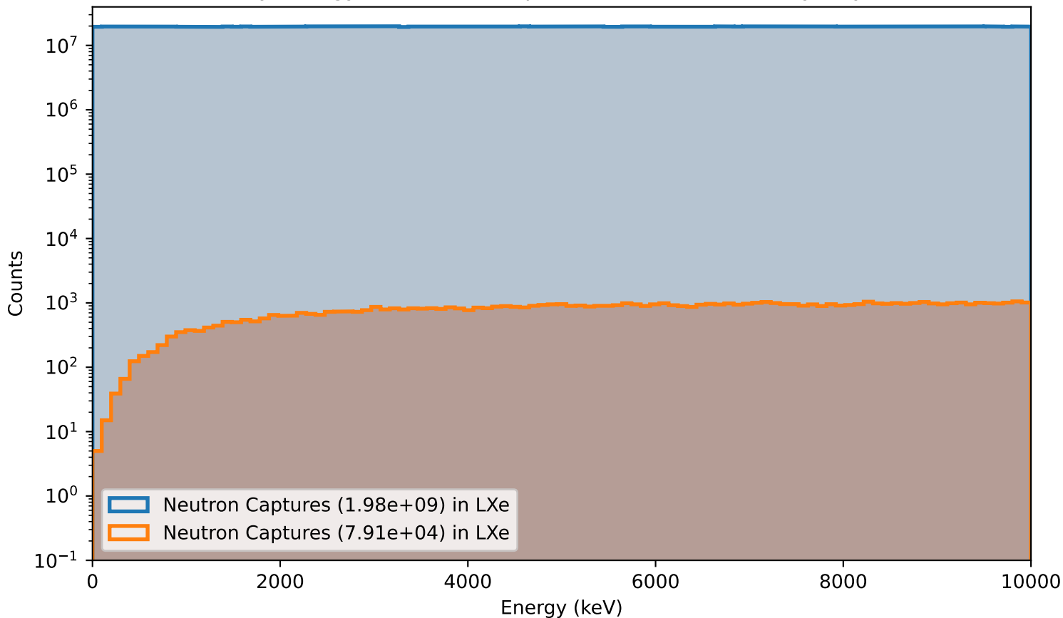
Primary energy of Neutron Captures in LXe (10cm,Polyethylen25)
