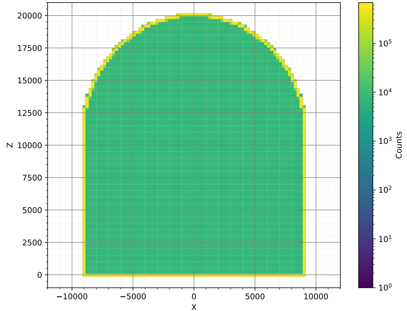
PrimaryNeutrons (10cm, Polyethylen25, 1.98e+08)
