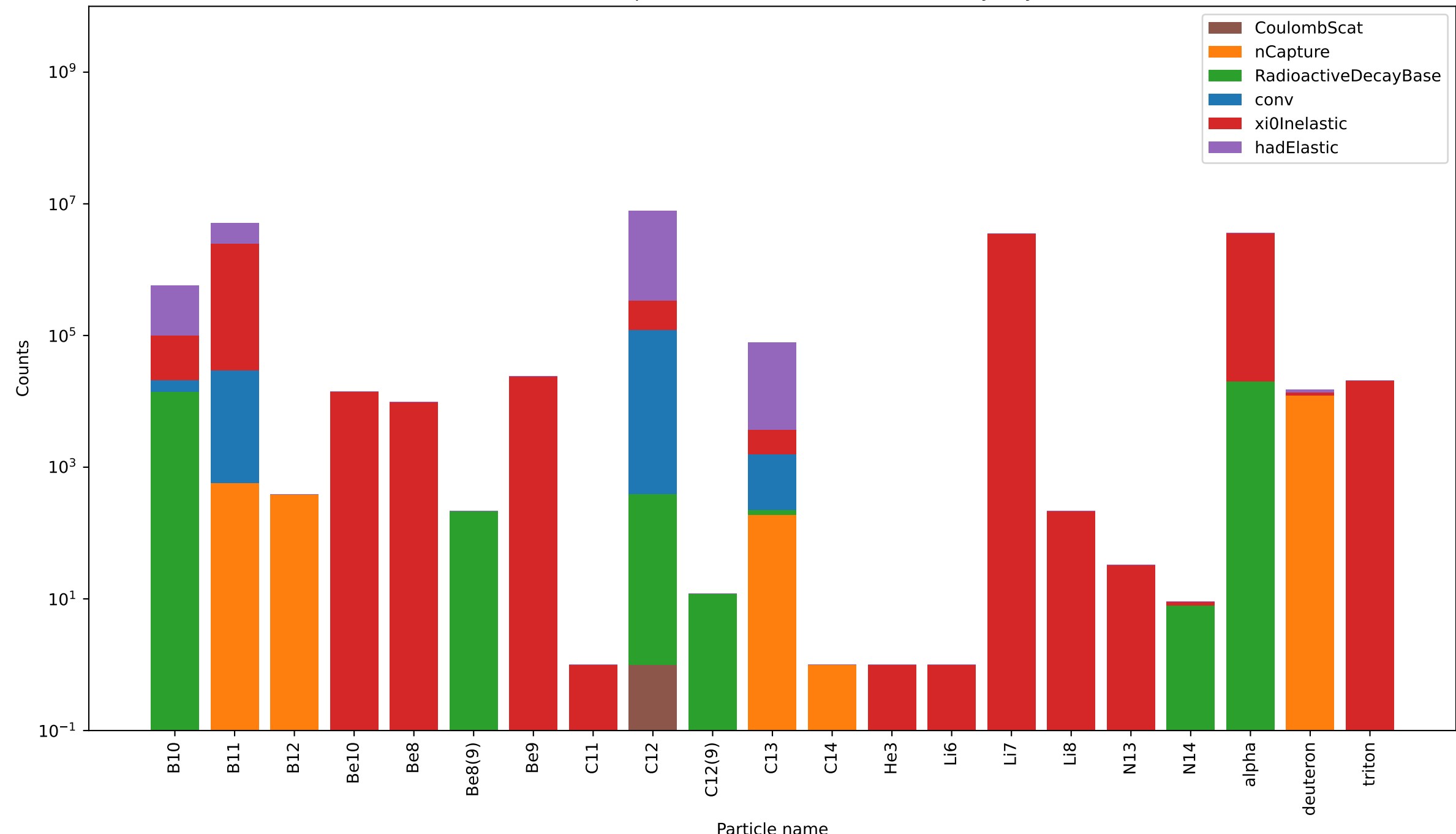
Neutron activation products in the Absorber (10cm Polyethylen25)
