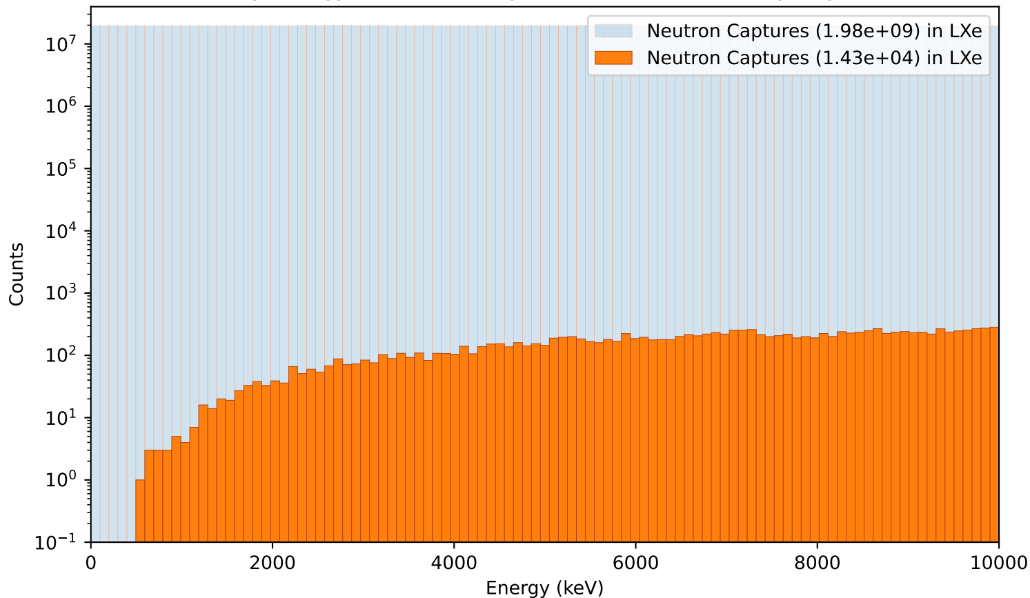
Primary energy of Neutron Captures in LXe (20cm,Polyethylen25)
