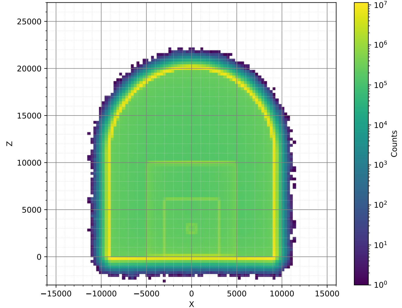
NeutronActivations (20cm, Polyethylen25, 2.43e+09)
