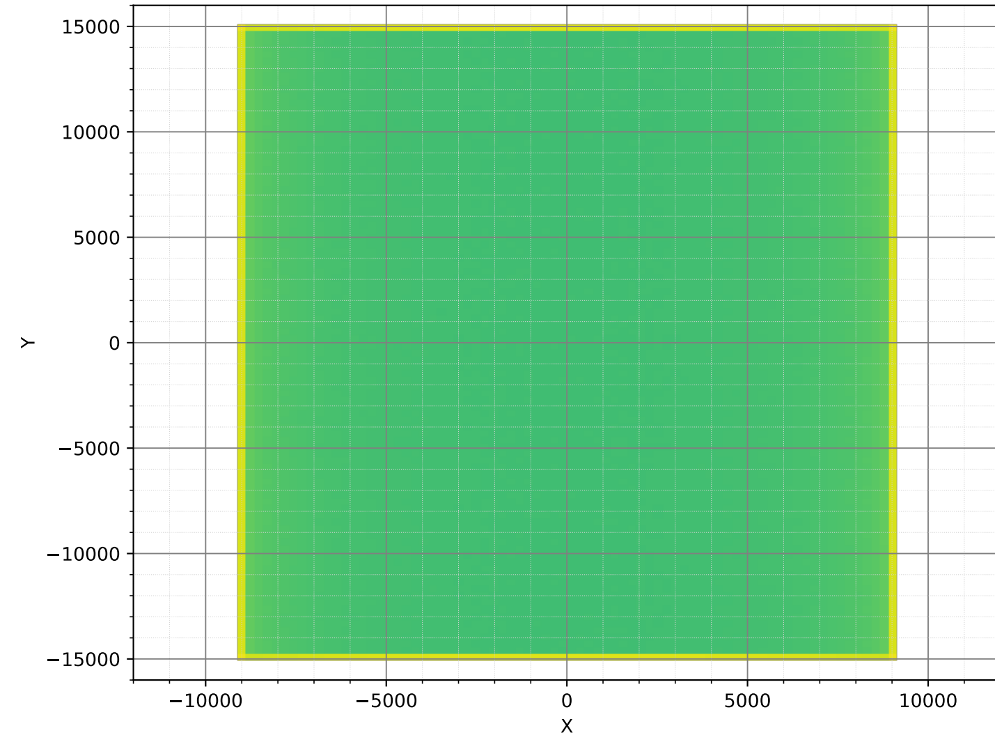
PrimaryNeutrons (20cm, Polyethylen25, 1.98e+08)
