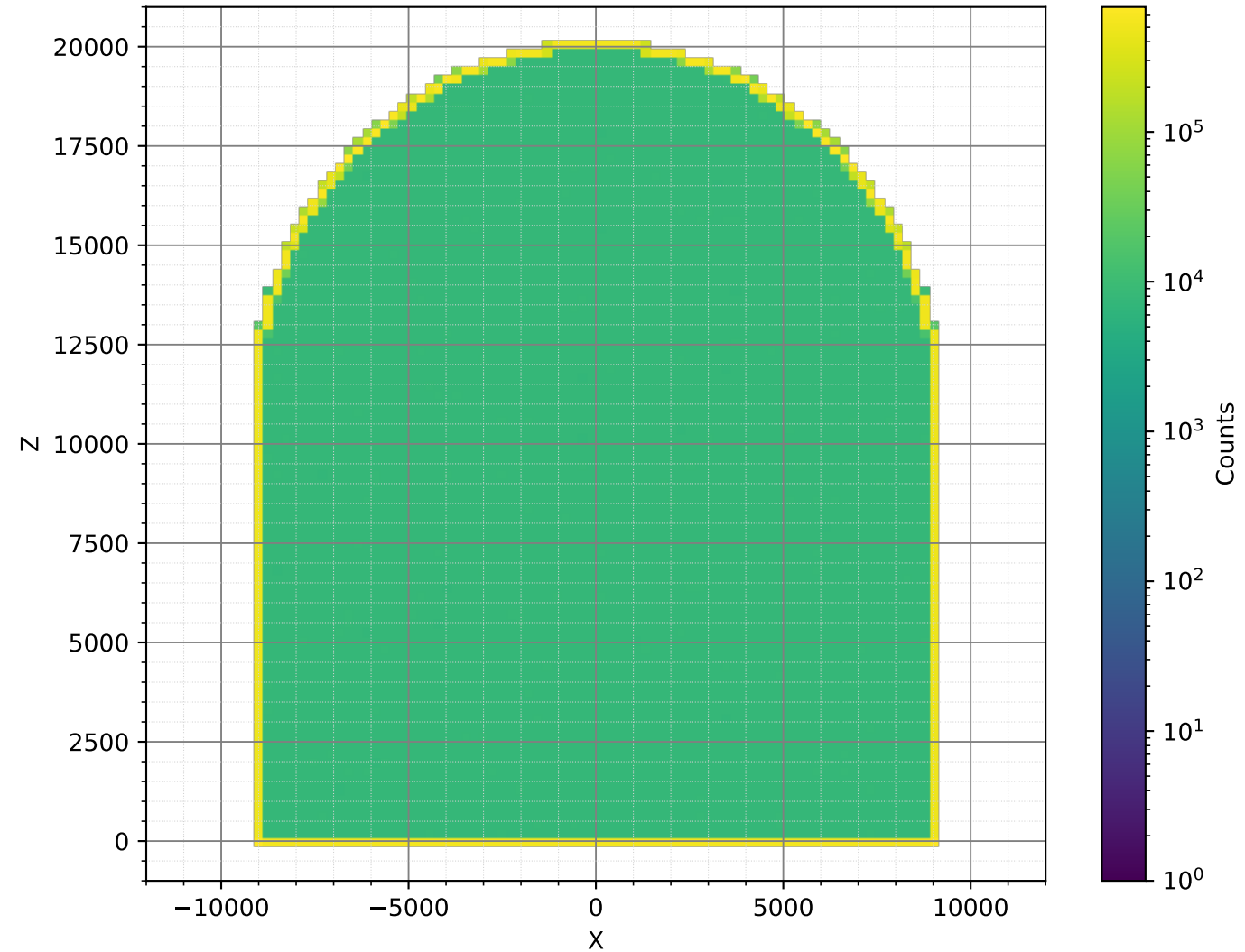
PrimaryNeutrons (20cm, Polyethylen25, 1.98e+08)
