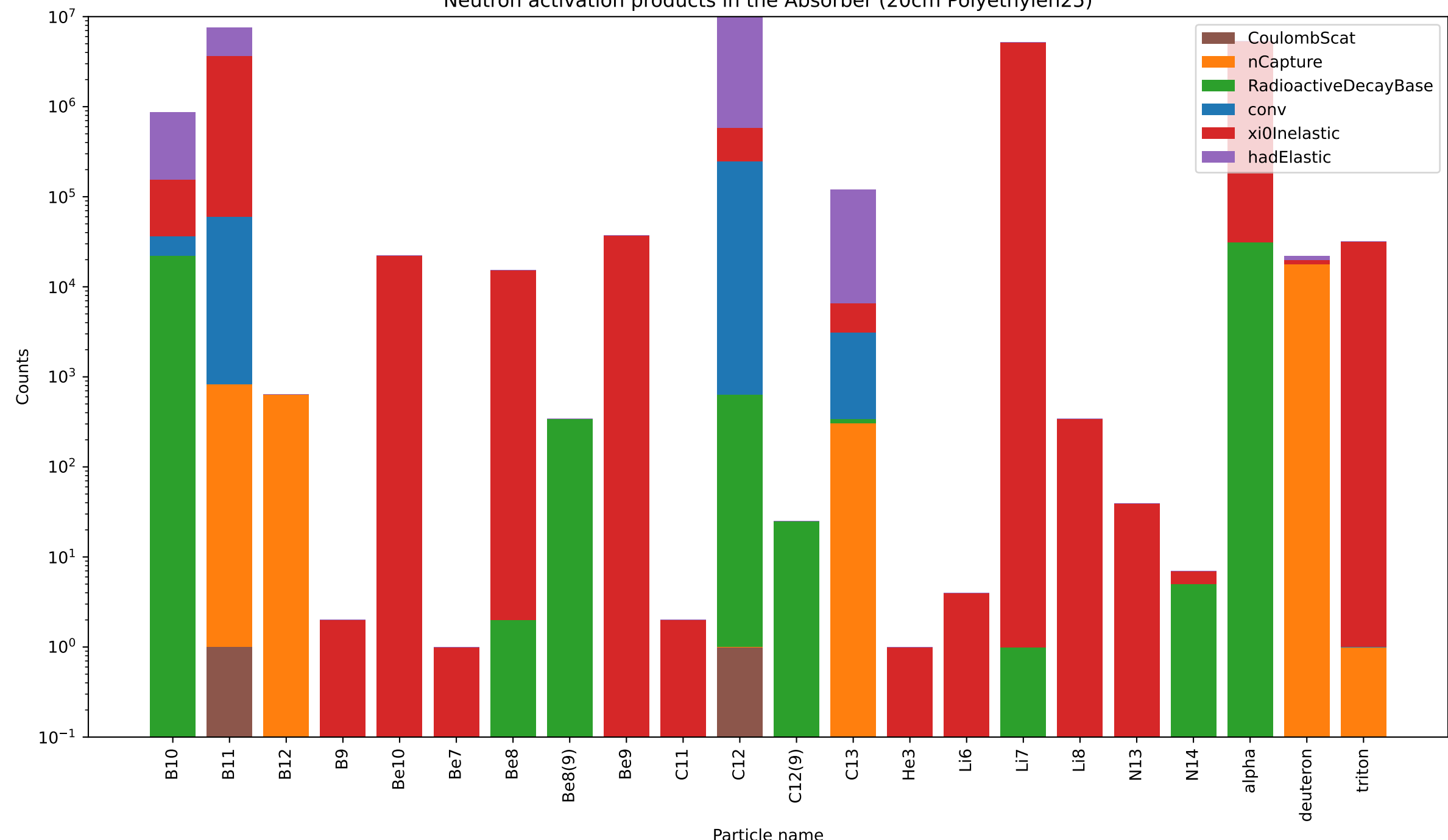
Neutron activation products in the Absorber (20cm Polyethylen25)
