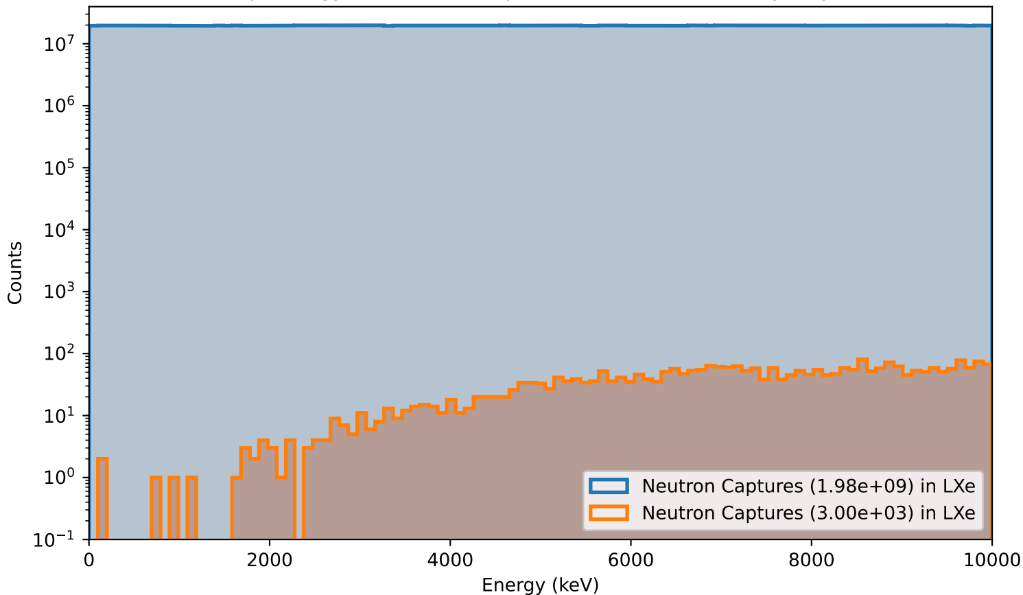
Primary energy of Neutron Captures in LXe (30cm,Polyethylen25)
