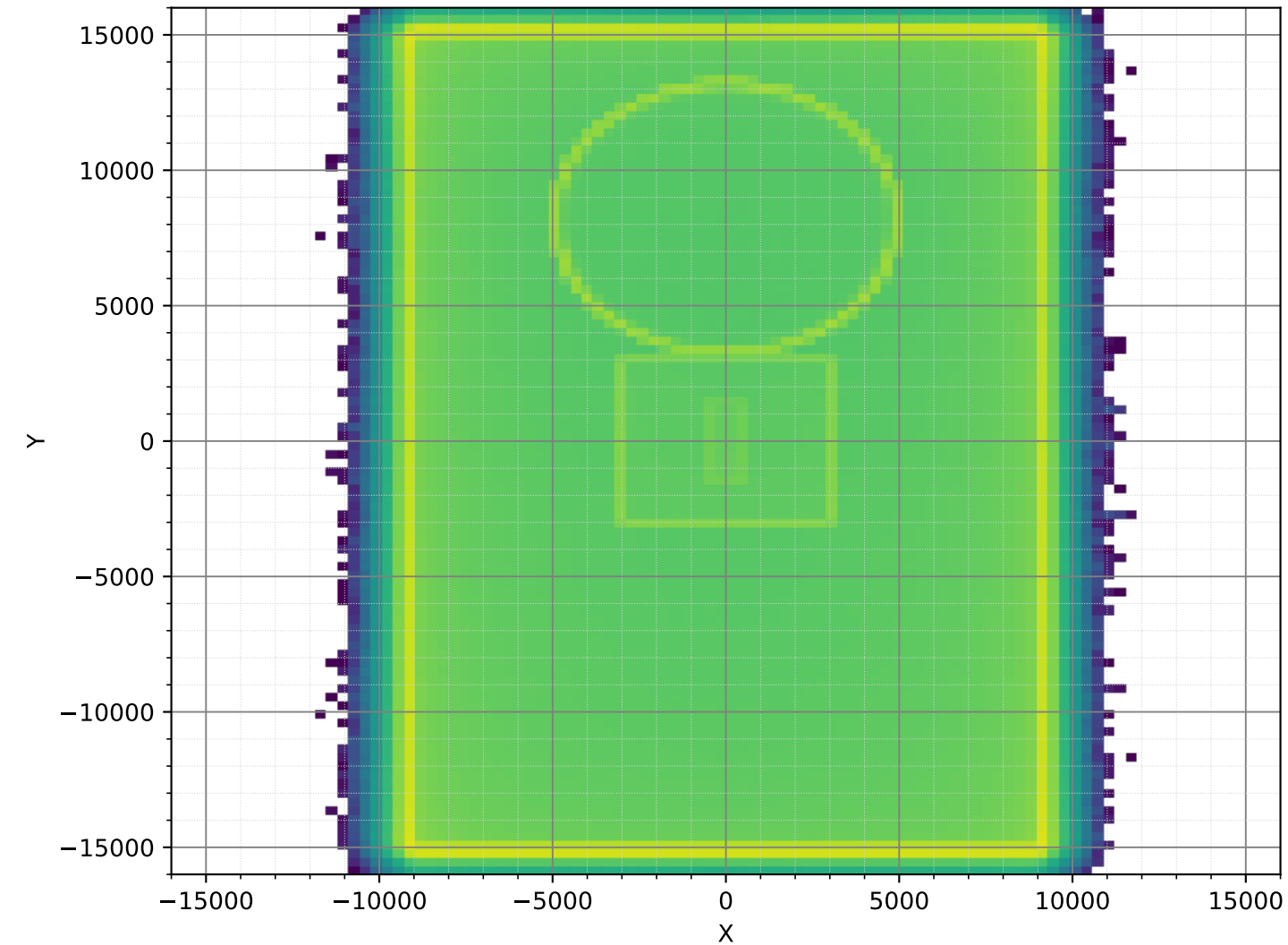
NeutronActivations (30cm, Polyethylen25, 2.43e+09)
