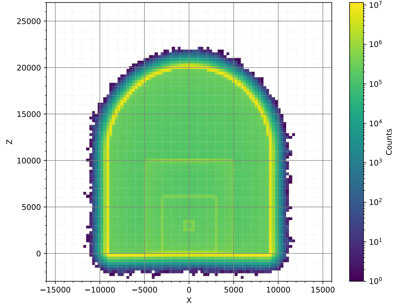
NeutronActivations (30cm, Polyethylen25, 2.43e+09)
