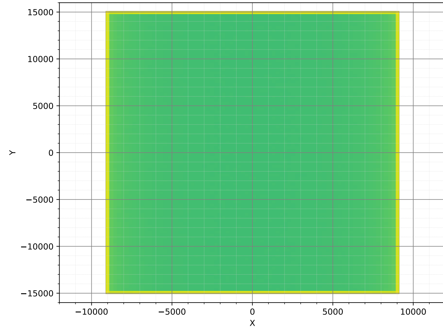
PrimaryNeutrons (30cm, Polyethylen25, 1.98e+08)
