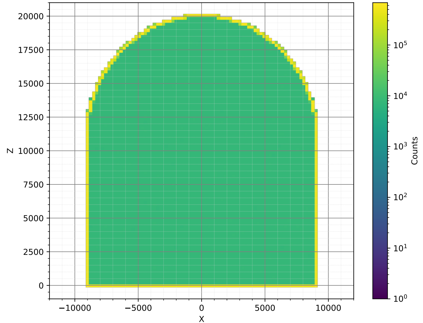
PrimaryNeutrons (30cm, Polyethylen25, 1.98e+08)
