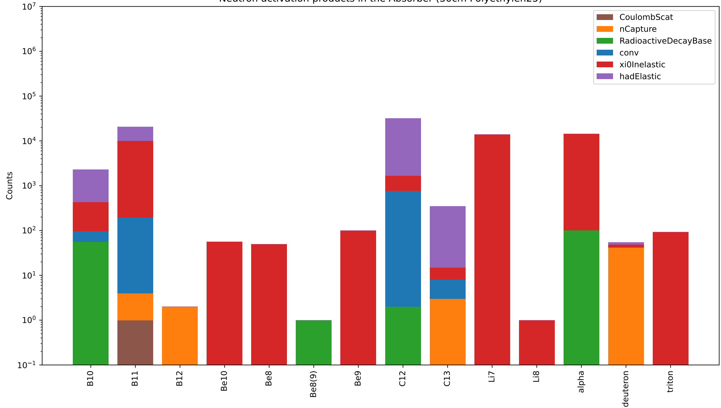
Neutron activation products in the Absorber (30cm Polyethylen25)
