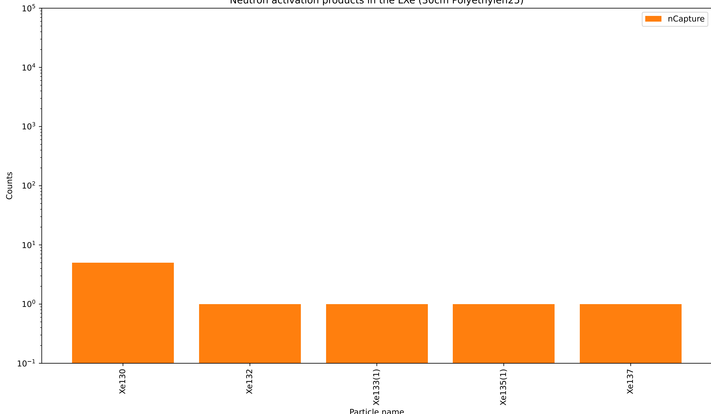
Neutron activation products in the LXe (30cm Polyethylen25)
