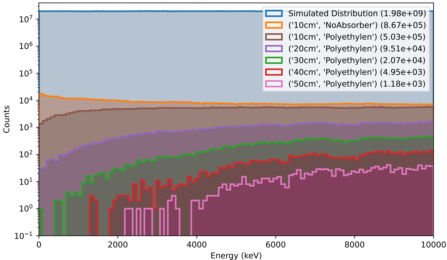
Primary energy of Neutron Captures in LXe
