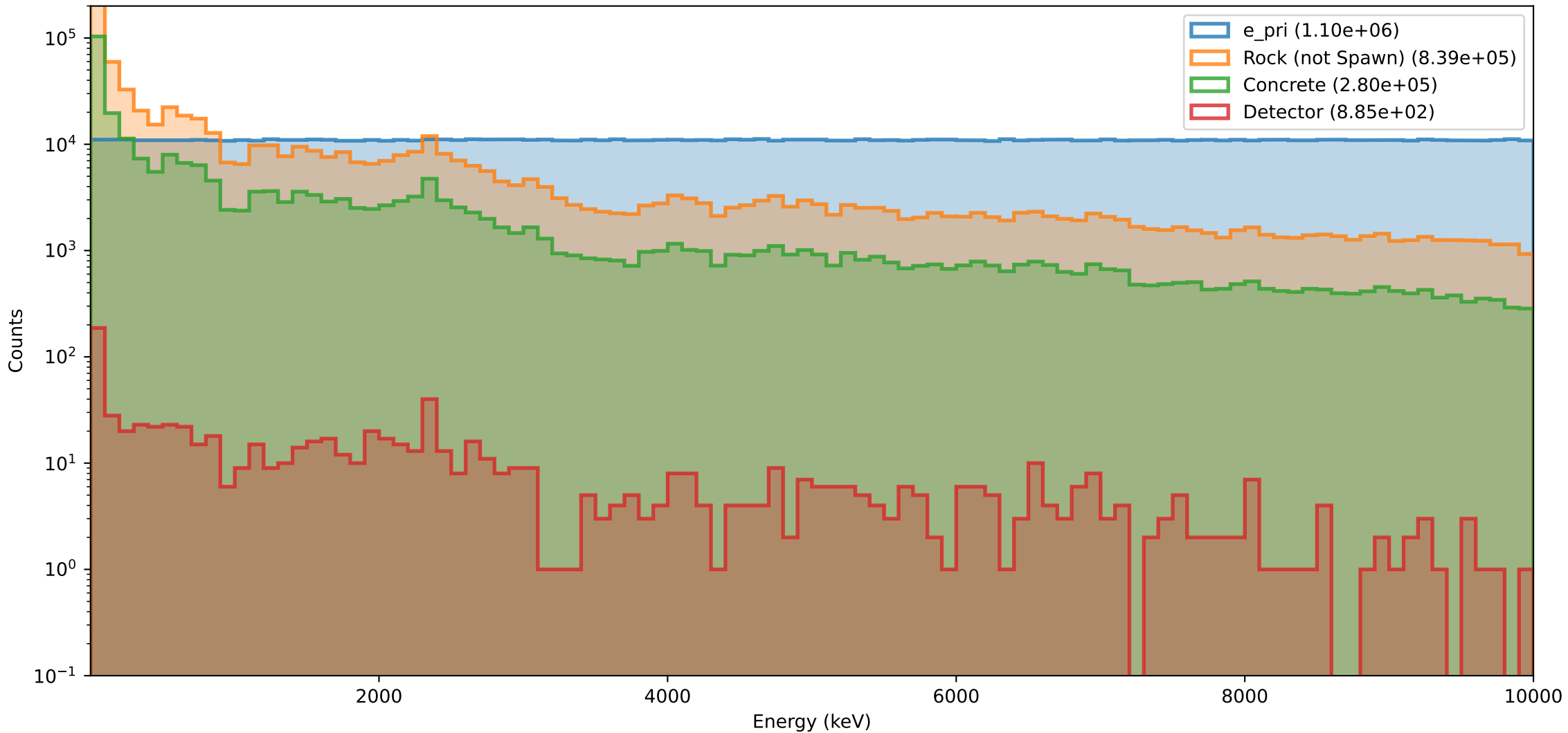
Energy distribution entering different volumes (XeSim bkoberg)
