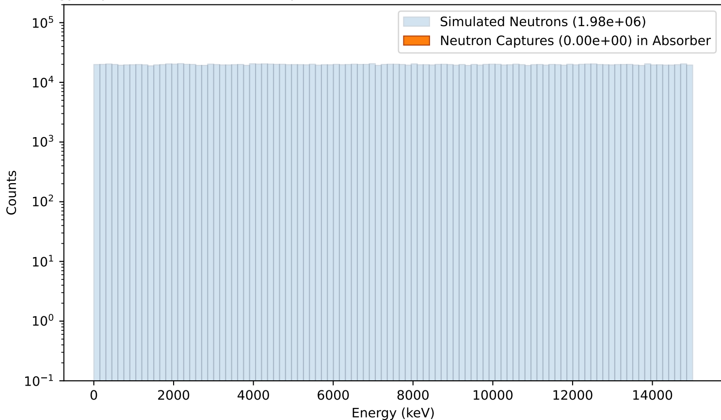
Energy dependence of Neutron Captures in the Absorber (50cm,NoAbsorber,ThreeLXeVolum
