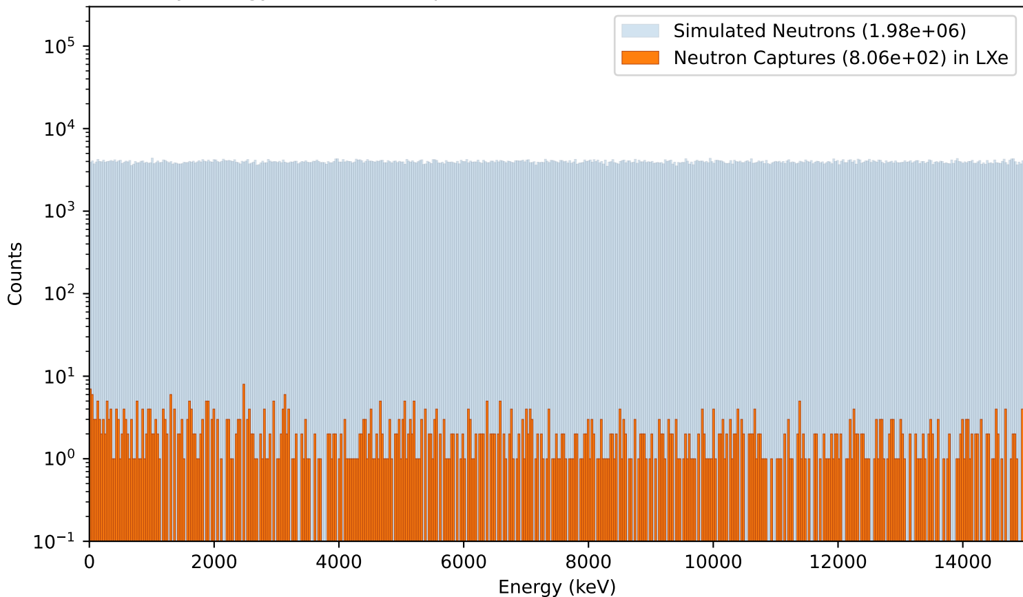
Primary energy of Neutron Captures in LXe (50cm,NoAbsorber,ThreeLXeVolumes)
