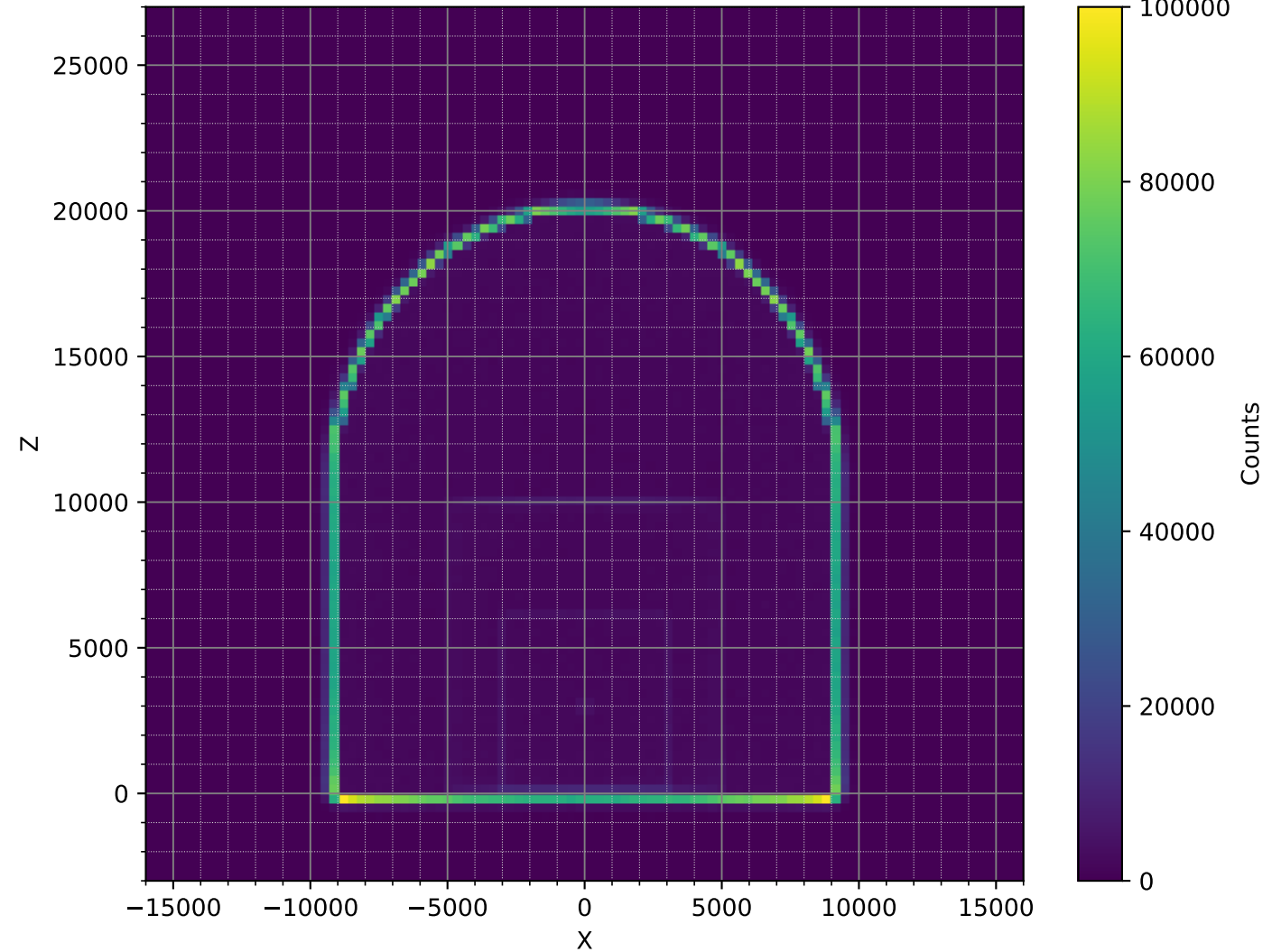
XZ-Projection of NeutronActivations (50cm, NoAbsorber, ThreeLXeVolumes)
