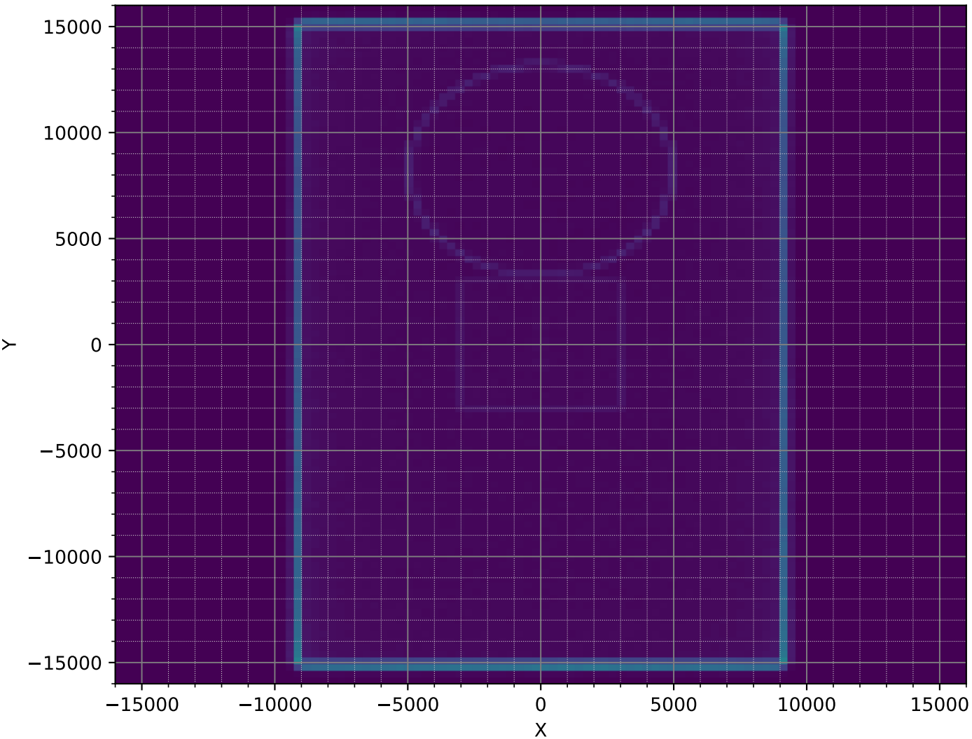
XY-Projection of NeutronActivations (50cm, NoAbsorber, ThreeLXeVolumes)
