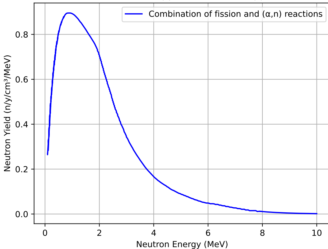
Neutron Yield of 0.84 ppm ^{238}\text{U} + 2.45 ppm ^{232}\text{Th}
