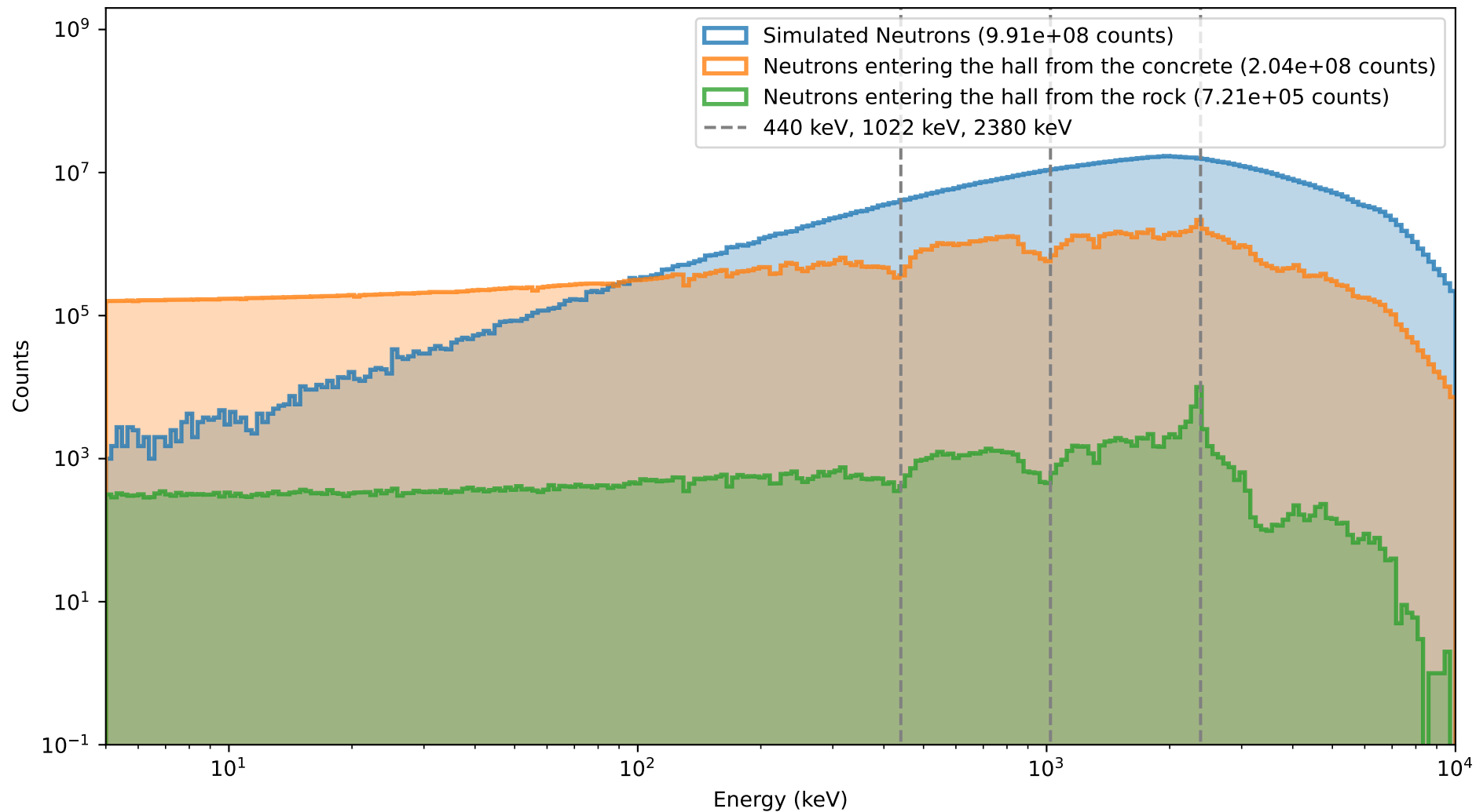
Distribution of neutrons with specific energy reaching the count volume
