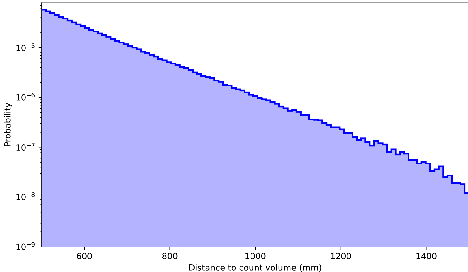
Neutrons probability of reaching the count volume with distance x ( 9.93\text{e}+08 events)
