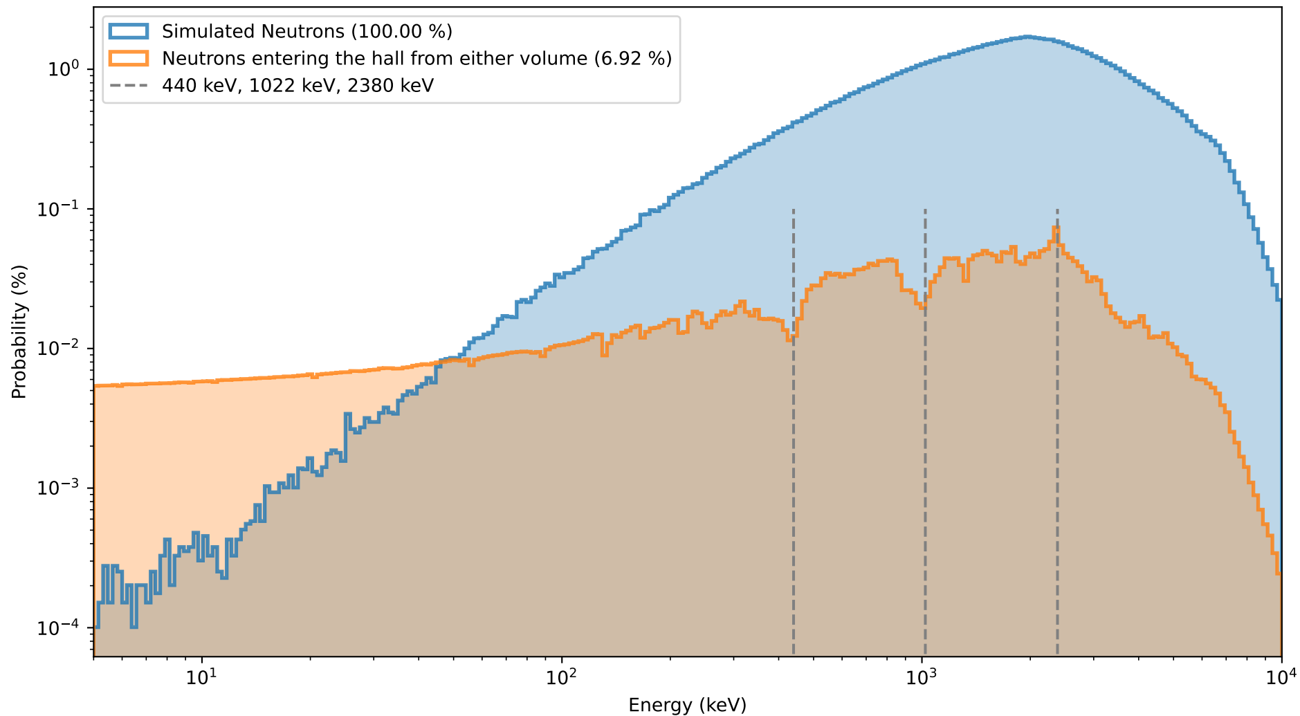
Combined probability distribution of neutrons with specific energies reaching the count volume
