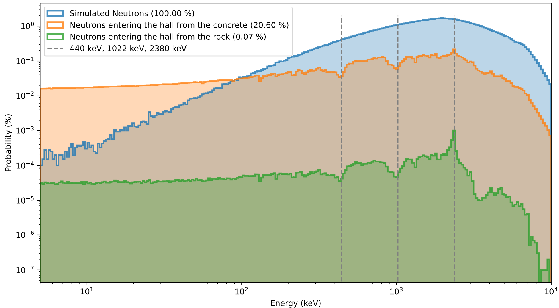
Probability distribution of neutrons with specific energies reaching the count volume
