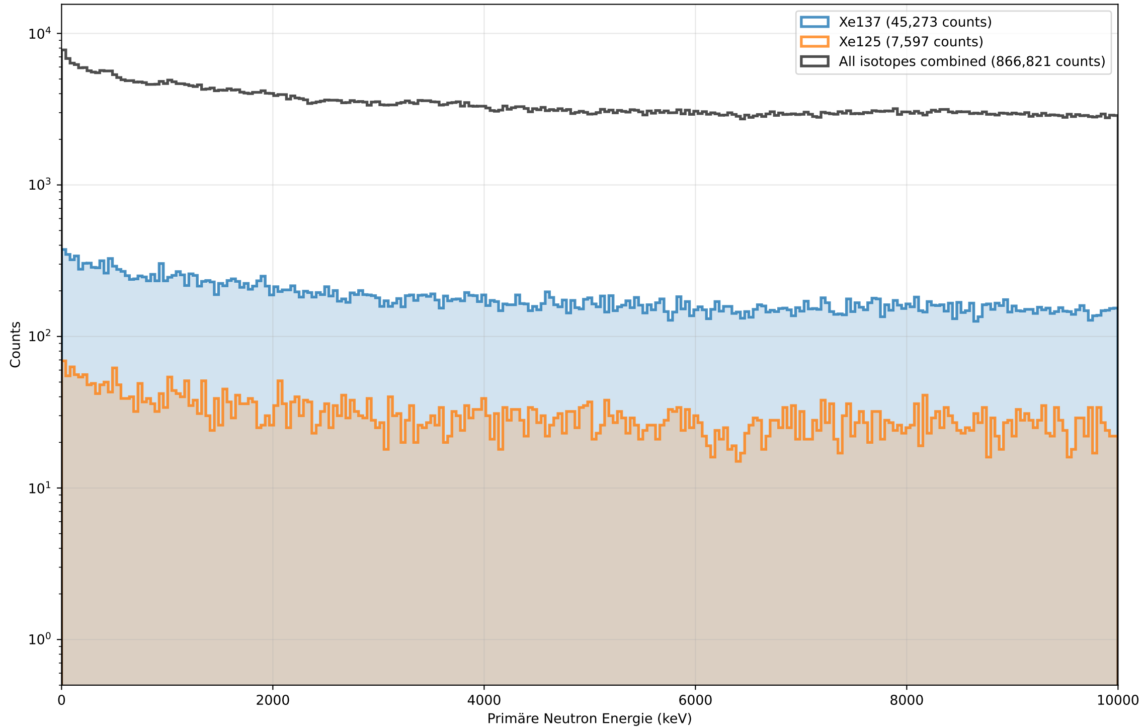
Primary energy dependent neutron captures in LXe
