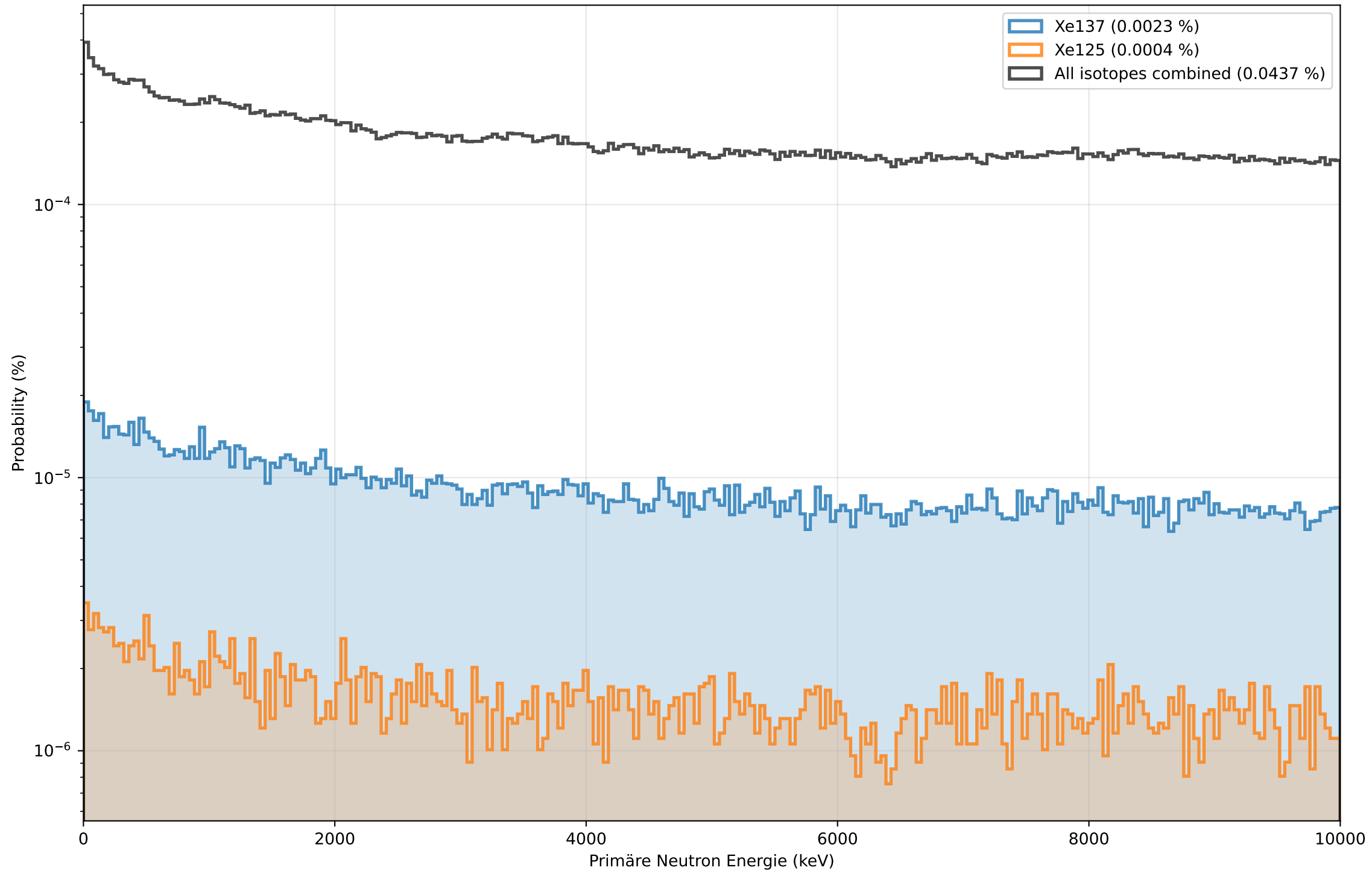
Probability of neutron captures in LXe with different primary energies using no absorber
