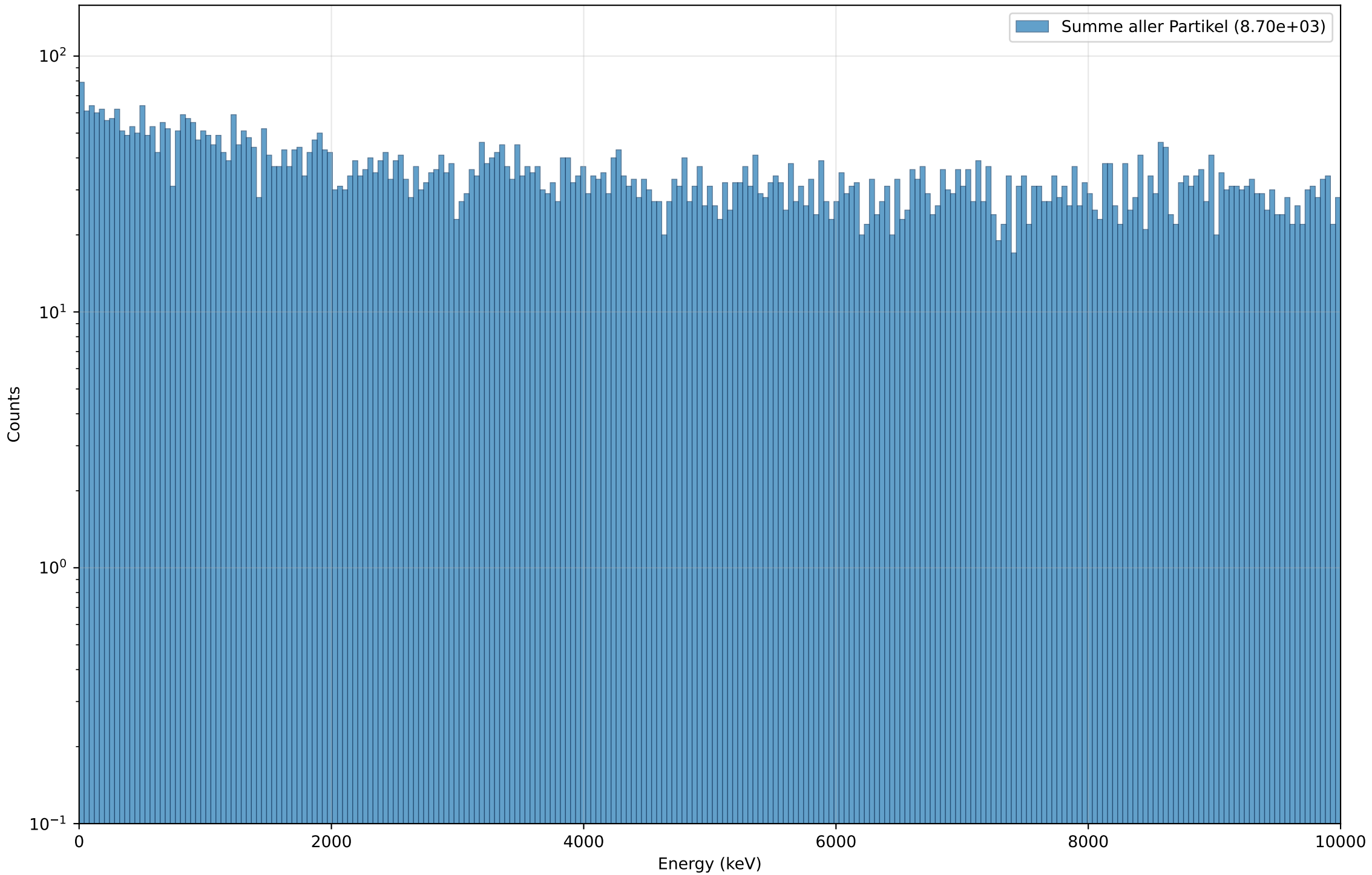
Summe aller Neutron Capture Energien in LXe (10cm, NoAbsorber)
